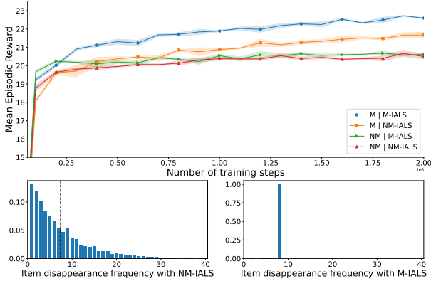
Figure 6. Top: Learning curves of agents with (M) and without memory (NM) trained on M-IALS and NM-IALS. Bottom: item disappearance frequencies with NM-IALS and with M-IALS.
