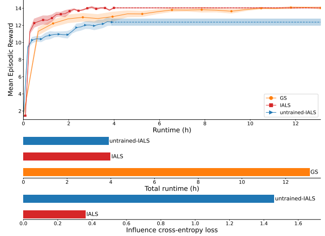
Figure 5. Top: Learning curves of agents trained with the GS, the IALS and the untrained-IALS on the warehouse environment as a function of wall-clock time. The dotted horizontal lines at the end of the red and blue curves show the final performance of the agents after 2M timesteps of training. Middle: Total runtime of training for 2M steps on the three simulators. Bottom: Cross entropy loss for the trained and untrained AIPs.
