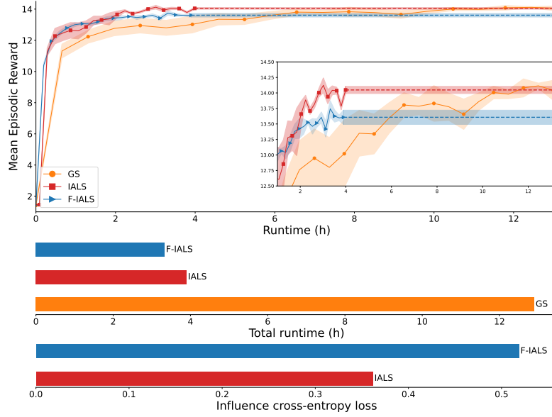
Figure 13. Top: Learning curves of agents trained with the GS, the IALS and the F-IALS on the warehouse commissioning task as a function of wall-clock time. Zoom in version of the same chart showing the performance difference between IALS and F-IALS. The dotted horizontal lines show the final performance of the agents after 2M timesteps of training. The dotted horizontal line at the beginning of the red curve corresponds to the AIP training time. Second from the bottom: Total runtime of training for 2M steps on the three simulators. Bottom: Cross entropy loss for the two AIPs.
