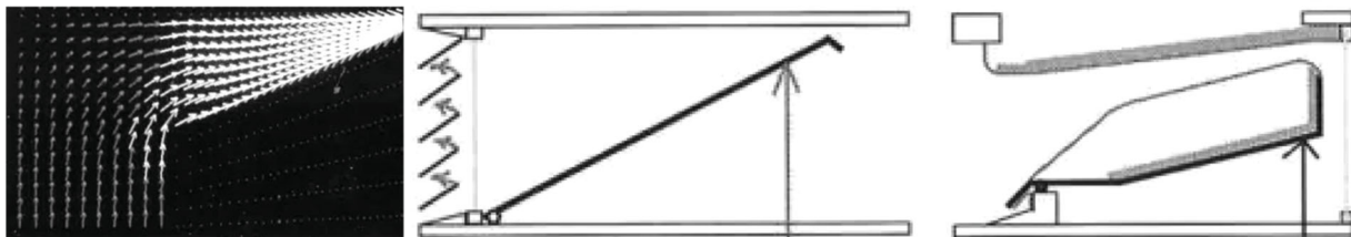
Figure 2. CFD-simulation of air flow in a venturi-shaped inlet (left) and two types of similar air inlets (right) that have been tested in a climate chamber. In the right model sound-absorbing materials are added. However, a venturi-shape in itself is not favourable for sound-isolation. A protecting element at the outside (like simulated in the CFD-calculation) could improve this. This way of protection does not have an effect on the air resistance.
