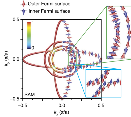
Figure 8. Calculated Fermi surface of the (001) \text{SrTiO}_3 surface showing the magnitude (left, in units of \hbar/2 ) and direction (right) of the spin. These calculations expose the spin angular momentum-kinetic momentum locking occurring at the Fermi surface for the different orbitals. For the circular d_{xy} subbands, we observe that the spins wind tangentially to the Fermi contour (i.e. the spins are aligned perpendicularly to the kinetic momentum), while for the elliptical d_{xz}/d_{yz} subbands they are aligned almost perpendicular to the Fermi contour (i.e. the spins are aligned perpendicularly to the dominant contribution of the kinetic momentum, k_y for the d_{yz} and k_x for the d_{xz} ). At the avoided crossing points (see the enlargement at the bottom right square), each subband splits for the two spin states, resulting in an effective Rashba-type spin-orbit interaction. Reprinted by permission from Nature, P. King et al. , Nat. Commun. 5 3414 (2014), Copyright (2014).
