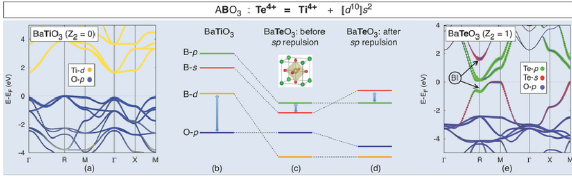
Figure 12. Concept of band inversion according to DFT calculations. (a),(b) The electronic structure of the band insulator ( Z_2=0 ) \text{BaTiO}_3 shows a gap between O-2p states and Ti-3d states (blue arrow); (c) replacing Ti with Te, the gap opens within the Te states, between the 5s and the 4p bands; (d),(e) considering the effect of sp repulsion, there is a band inversion (BI) and the formation of a topological insulator ( Z_2=1 ). This electronic structure is however strongly susceptible to atomic distortions that modify the cubic phase and suppress the band inversion. Reprinted from Ref. [81].
