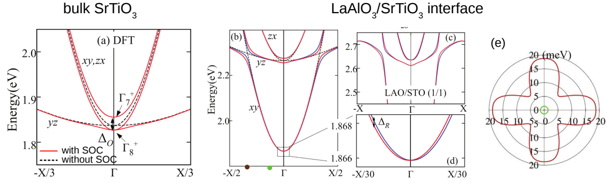
Figure 6. (a) Band structure of bulk \text{SrTiO}_3 obtained by DFT calculation without and with SOC. (b) Band dispersion for the \text{LaAlO}_3/\text{SrTiO}_3 interface without (dashed line) and with (continuous lines) SOC and breaking of inversion symmetry. The blue and red colors differentiate the spin state. Zoom of the crossing region (c) and of the bottom of the band (d) with the spin-splitting \Delta_R induced by the breaking of inversion symmetry (Rashba SOC). (e) Angular dependence of the spin splitting at the bottom of the d_{xy} band (green line referring to the green point in (b)) where it is Rashba SOC and at the d_{xy} - d_{yz}/d_{zx} crossing region (brown). Reprinted with permission from Z. Zhong et al. , Phys. Rev. B 87 , 161102 (2013). Copyright (2013) by the American Physical Society.
