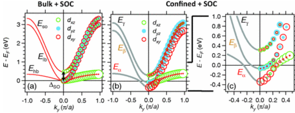
Figure 9. Tight-binding calculations for KTaO 3 bulk with spin-orbit coupling (SOC) and surface with SOC (Confined + SOC). The weight of the d_{xz} , d_{yz} and d_{xy} orbital symmetry in each band/subband is proportional to the size of the circles. Reprinted with permission from A. Santander-Syro et al. , Phys. Rev. B 86 , 121107 (2012). Copyright (2012) by the American Physical Society.
