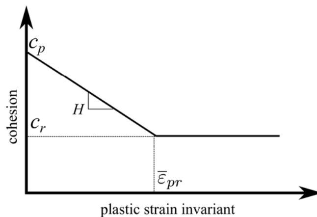
Fig. 1. Schematic of the strain-softening constitutive model [2].
