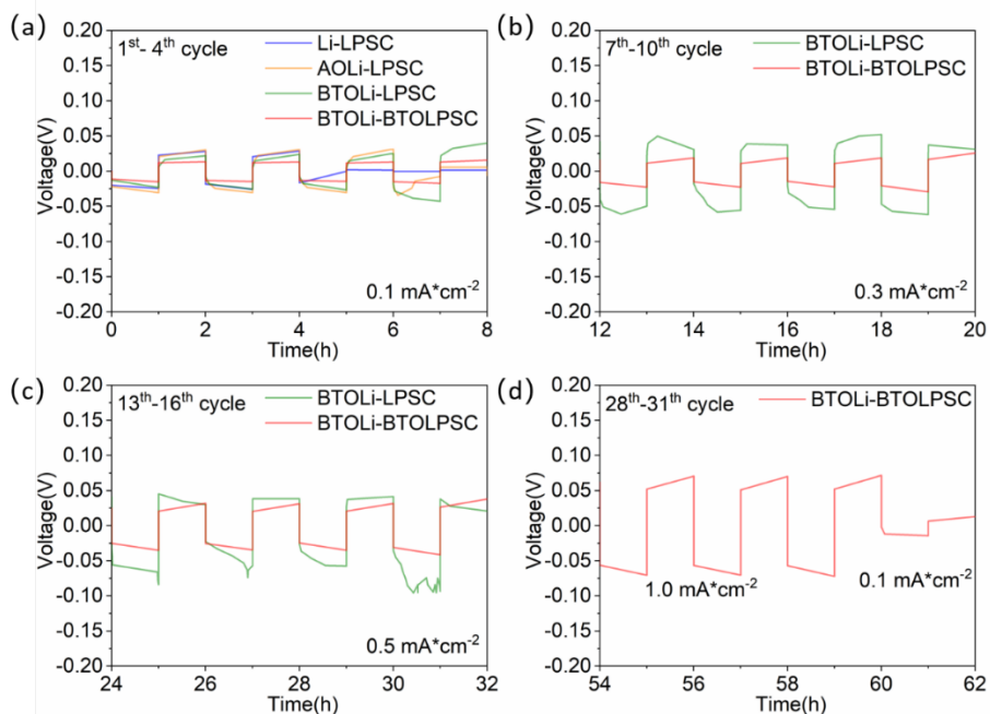
Figure S3.5 Detailed voltage profiles of rate performance using bare Li electrode, BTOLI or AOLI composite electrodes and LPSC or BTOLPSC electrolytes at different cycles.
