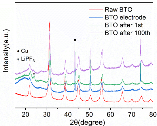
Figure S2.9 XRD patterns of BTO raw material and BTO electrodes before and after 1 st and 100 th cycles.
