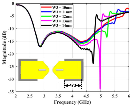
Fig. 10: Effect of passive and W3 on the |S_{11}| parameter of the dipole antenna. (W3=13mm bandwidth 61.44%)
