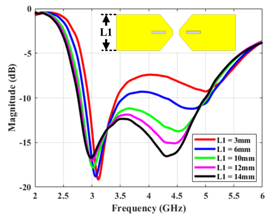
Fig. 6: Effect of L1 on the |S_{11}| parameter of the dipole antenna (L = 14mm bandwidth = %57.73).
