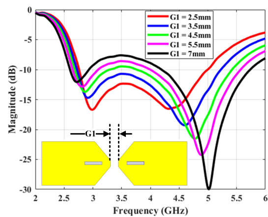
Fig. 7: Effect of G1 on the |S_{11}| parameter of the dipole antenna.
