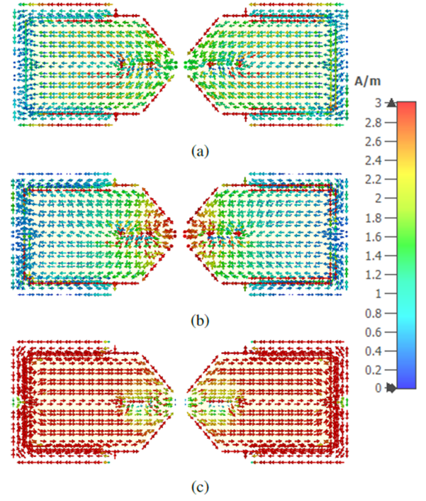
Fig. 9: Surface current of dipoles with passive elements at (a) 2.6 GHz (b) 3.6 GHz (c) 5 GHz.
