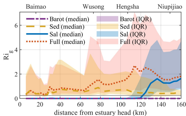
Figure 10. Modeled longitudinal changes (red dashed line in Figure 2) of the median and interquartile range (IQR) of the maximum gradient Richardson number Ri_g over the water column from January 1, 2007 to January 1, 2008 in the scenarios of Barot (purple), Sed (yellow), Sal (blue), and Full (red) (scenarios see Table 2). The values over 0.25 (gray solid line) suggest more stratification effect. The estuary head is at Xuliujing (see also Figure 2).
