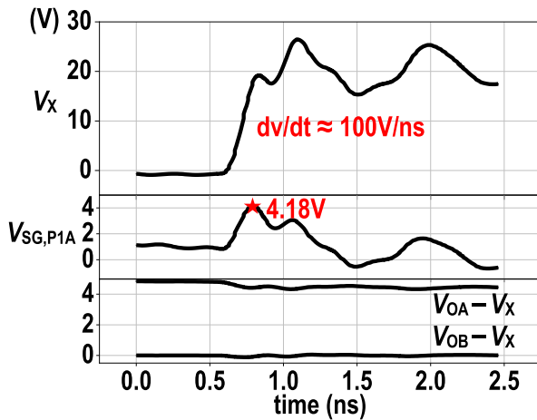
Fig. 8. Post-layout simulation results when dv/dt \approx 100\text{V/ns} .
