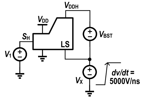
Fig. 9. Testbench of the proposed level shifter under dv/dt = 5000\text{V/ns} .
