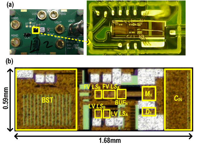
Fig. 16. (a) PCB photos, and (b) chip micrograph.
