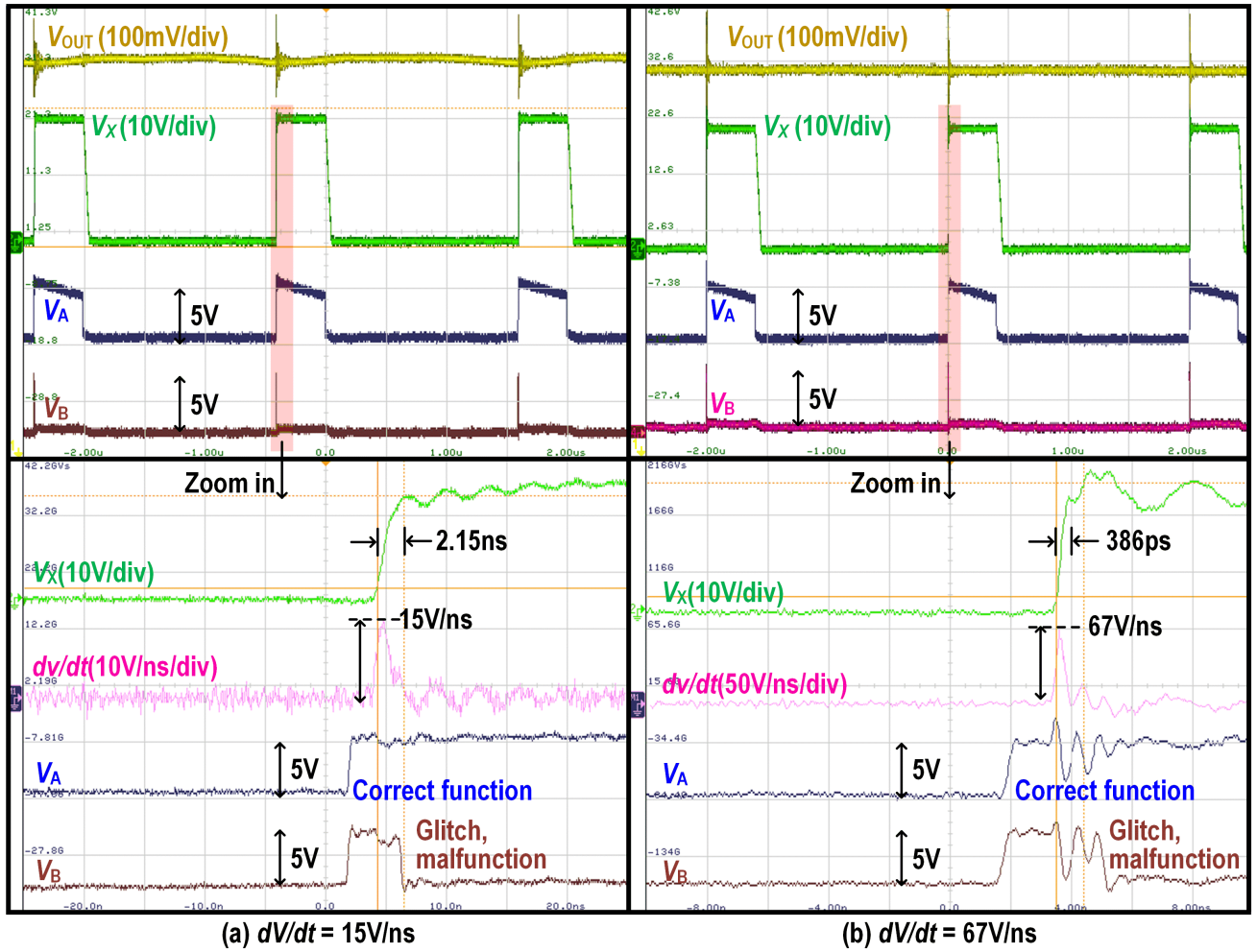
Fig. 17. Measured steady-state waveforms (a) with a 15V/ns, and (b) a 67V/ns dv/dt .
