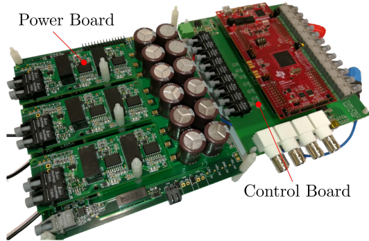
Fig. 3. Power, gate driver and control boards of the remote laboratory setup.
