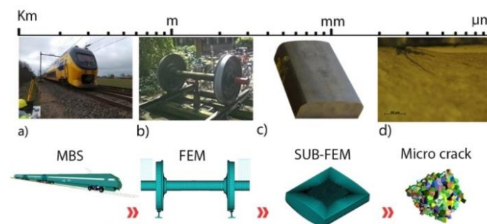
Figure 32. Schematic graph of multi-scale strategy for wheel-rail interaction [54]. a) Complete macro scale –vehicle/train
