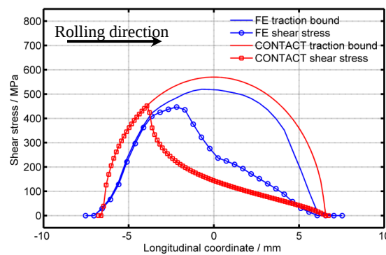
Figure 8. 2D surface shear stress slice plot.
