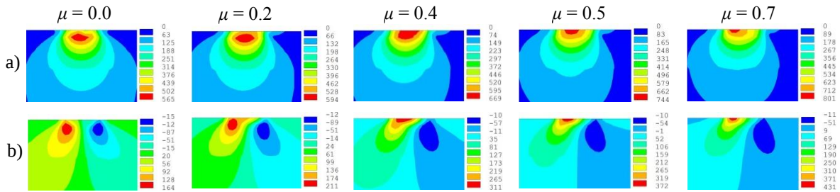
Figure 15. Sub-surface stress distribution (Unit: MPa). a) Von Mises stress; b) Shear stress.
