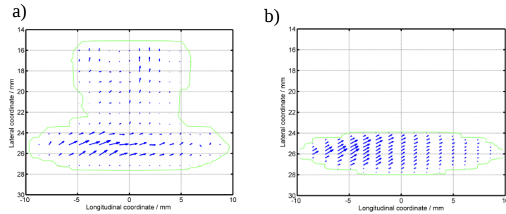
Figure 25. Surface shear stress quiver plot at the lateral shift of -5.5mm. a). FE solution; b) CONTACT solution.
