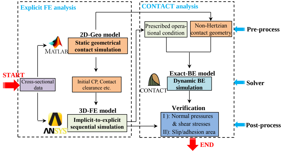
Figure 3. Integration procedure of CONTACT with FE model.
