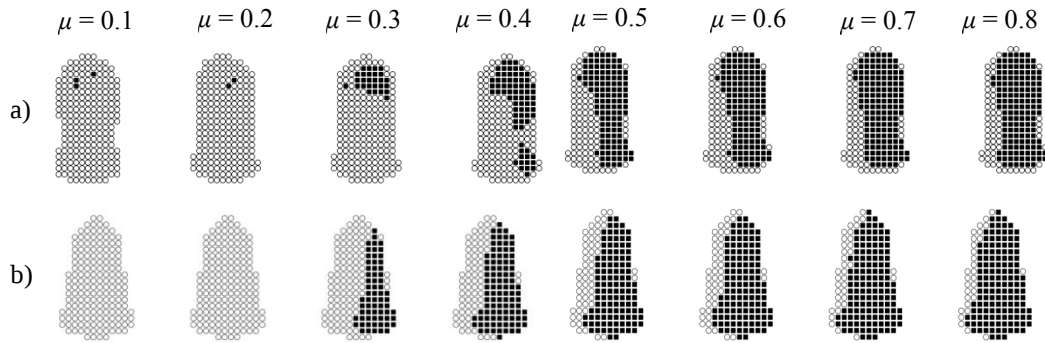
Figure 14. Slip-adhesion plot. a) FE solution; b) CONTACT solution. (Note: ○ refers to slip, ■ denotes stick).
