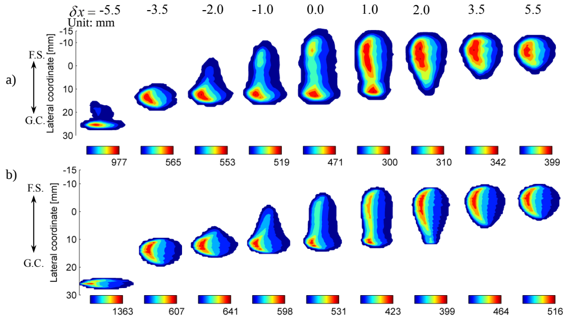
Figure 24. Shear stress distribution (Unit: MPa). a) FE solution; b) CONTACT solution.
