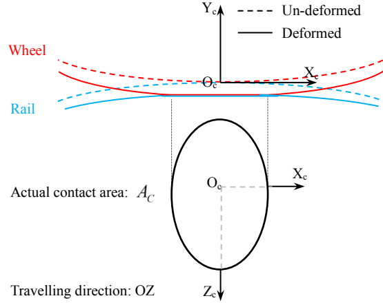
Figure 2 Schematic diagram of wheel-rail interaction in CONTACT (adapted from [28]).
