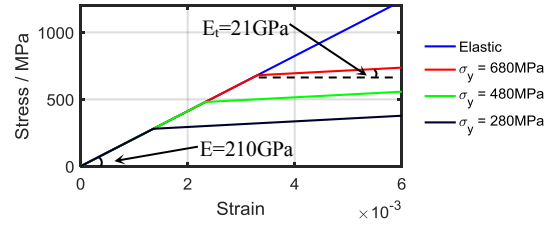
Figure 27. Schematic graph of the resulting bilinear elastic-plastic material model from the varying yield strength \sigma_y .
