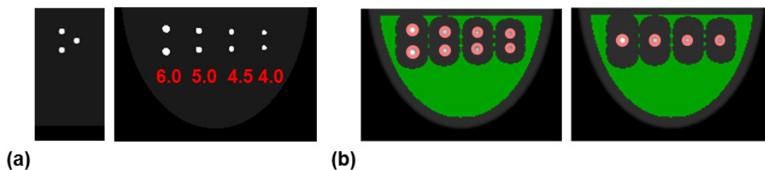
Figure 4. Slices through the breast phantom (a) left: slice parallel to sagittal plane through the 6.0 mm lesions, right: transverse slice at depth of two lesions. Lesion sizes indicated. (b). Transverse slices with red circles indicate the regions-of-interest used to determine the tumour signal while the green area denotes the background region.
