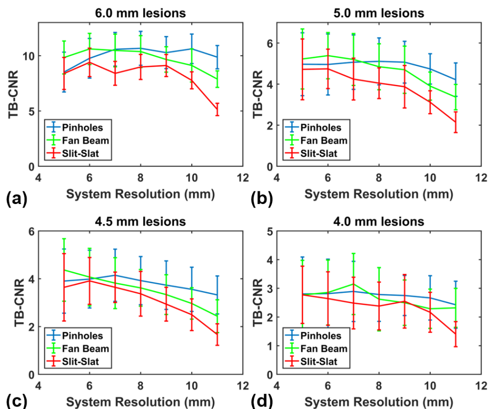
Figure 8. Plot of the TB-CNR as function of system resolution, where the TB-CNR is obtained as the maximum over iterations 5–32 and Gaussian filters with 0–10 mm FWHM as indicated in tables 3–5. The different lines represent the different collimator types and results are shown for (a) 6.0 mm lesions, (b) 5.0 mm lesions, (c) 4.5 mm lesions and (d) 4.0 mm lesions.
