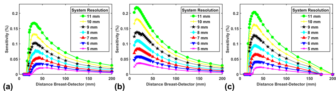
Figure 5. Sensitivity (averaged over the breast) for (a) pinhole, (b) fan beam, (c) slit-slat collimators as function of distance between detector and breast with the lines indicating different fixed system resolutions (5, 6, 7, 8, 9, 10, and 11 mm).
