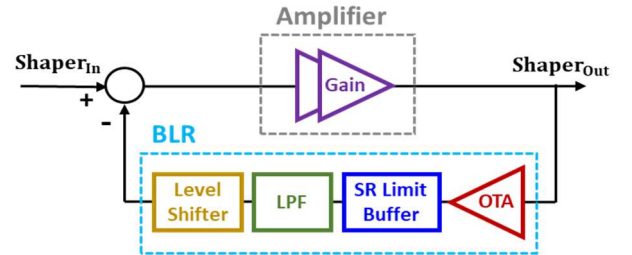
Fig. 4. Block diagram of the signal shaper block.
