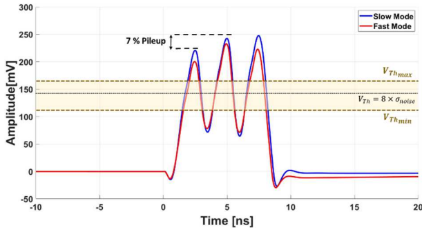
Fig. 11. Voltage signals after the signal shaper block for three consecutive trigger pulses and C_{LPP} = 500 fF for a high gain CSA programmed in slow (blue line) and fast (red line) modes.
