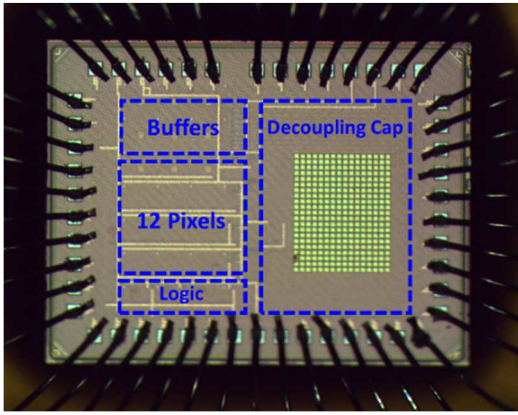
Fig. 8. Chip micrograph including 12 pixels, buffers, logic, and decoupling capacitors.
