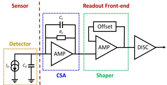
Fig. 1. Simplified block diagram of the readout frontend electronics.
