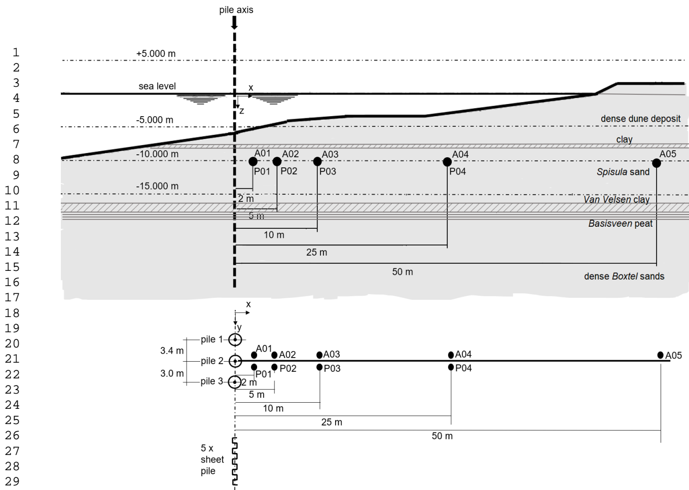
Fig. 1. Cross-section of test site and top view with monitoring equipment.
