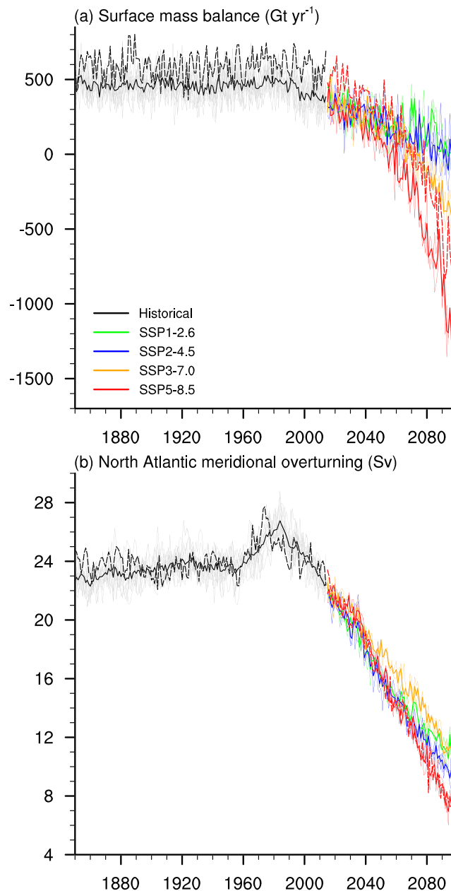
Figure 4. Comparison of evolution of (a) SMB ( \text{Gt year}^{-1} ) and (b) NAMOC index (Sv) for the historical (black, dashed) and SSP5-8.5 (red, dashed) coupled simulations in this paper versus CESM2.1 historical (black, solid) and scenario simulations (solid) with a prescribed surface elevation, nondynamical Greenland Ice Sheet (that is, with nonevolving CISM2.1). Thick lines represent CESM2.1 scenario ensemble means.
