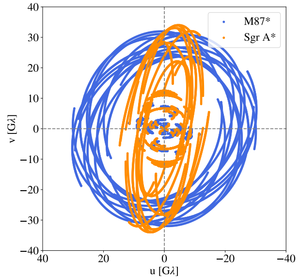
Fig. 2: An "ideal" (u, v) coverage for M87* and Sgr A* achieved by BHEX in the reference orbit. Observation conducted with ground array depicted in Fig. 1, at a frequency of 320 GHz, over 24 hours.
