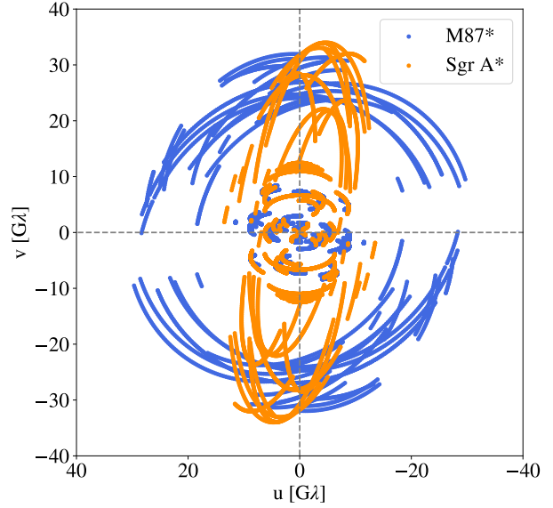
Fig. 8: 24 hour (u,v) coverage of M87* and Sgr A* by BHEX on 1 st Jan and 1 st June, respectively. Observations limited to when an optical downlink with the ground is achievable. Terminal gimbal capability limited to \pm 70^\circ . 45.5% and 36.8% loss in coverage of M87* and Sgr A*, respectively.
