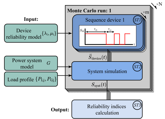
FIGURE 23. Proposed MC framework for reliability assessment of dc-SPSs.
