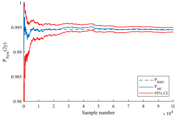
FIGURE 24. Simplified MC simulation for the propulsion subsystem with considering open circuit device failures with A_c = 0.9 and A_{r,i} = 0.95 .
