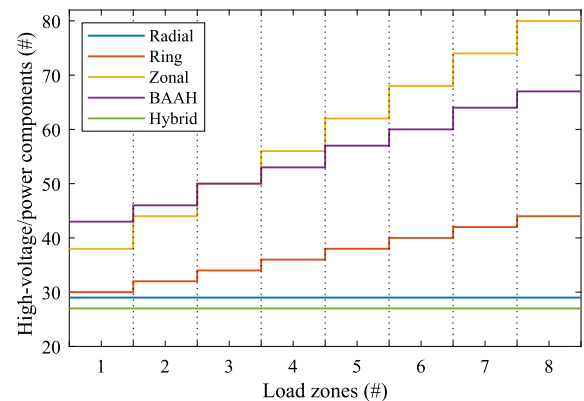
FIGURE 6. Comparison of the number of high-voltage high-power components for the five SPS topologies.
