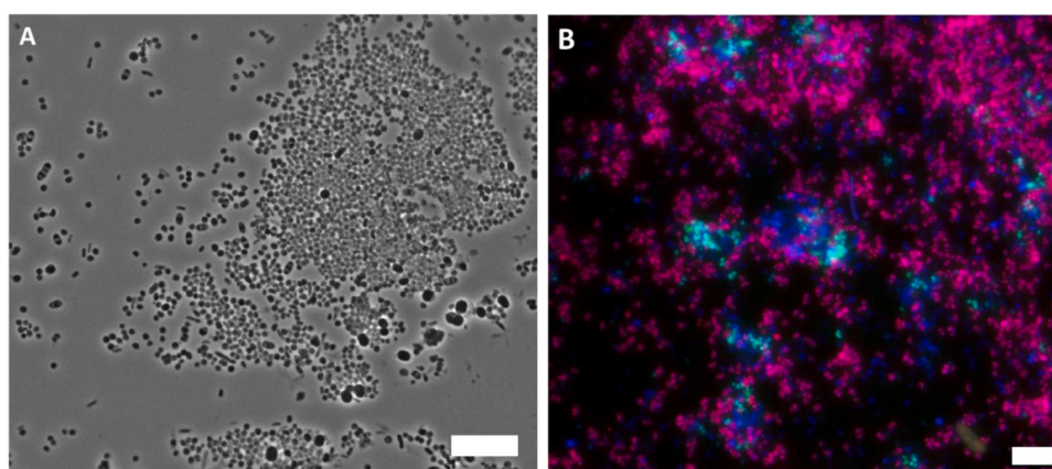
Fig. 6. Phase contrast and FISH picture of the microbial population. The scale bar is equal to 10 \mu\text{m} . Blue represents all microorganisms stained with probe EUBmix, magenta shows the PAO population stained with probe PAO651, and cyan shows the cluster stained with probe Tess644.
