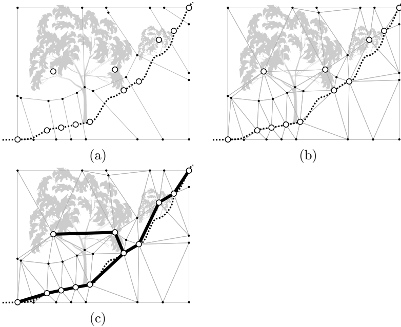
Figure 5.9: Labeling by crust. Voronoi diagram of original points (a), Delaunay triangulation of original and Voronoi points (b), connecting all original points joined by an edge (c).
