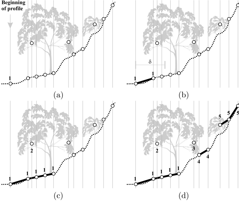
Figure 5.7: Consecutive point labeling. Move to beginning of label (a), label adjacent points (b), extend the label to other points (c), continue labeling unlabeled points (d)
