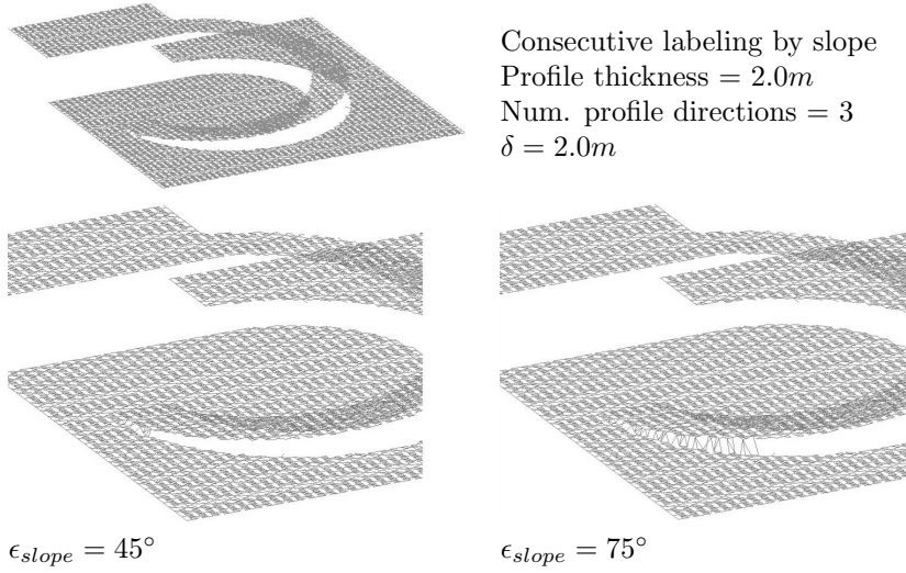
Figure 5.13: Segmentation example 2: Bridge connected to the bare earth (point spacing 1-1.4m).
