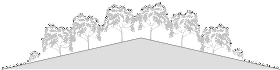
Figure 4.5: Zero ground returns. In the area covered by vegetation there are no hits off the bare earth
