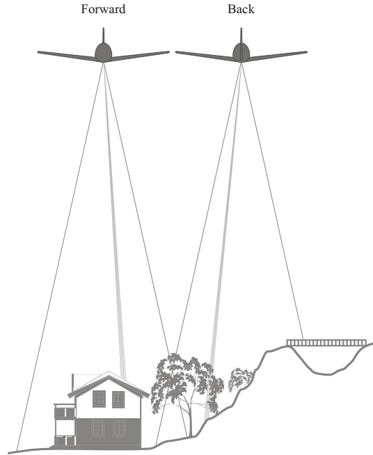
Figure 2.1: Airborne laser scanning. The landscape is scanned in strips, and the scans from the strips are combined to form a point cloud.
