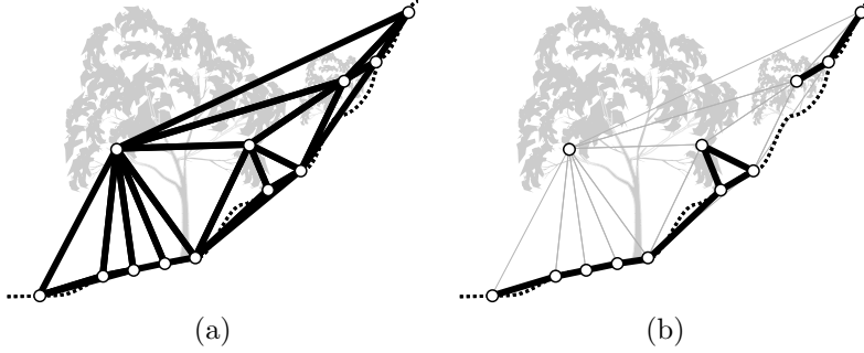
Figure 5.10: Labeling by proximity. Delaunay triangulation (a), removal of edges that are greater than a given weight (b).
