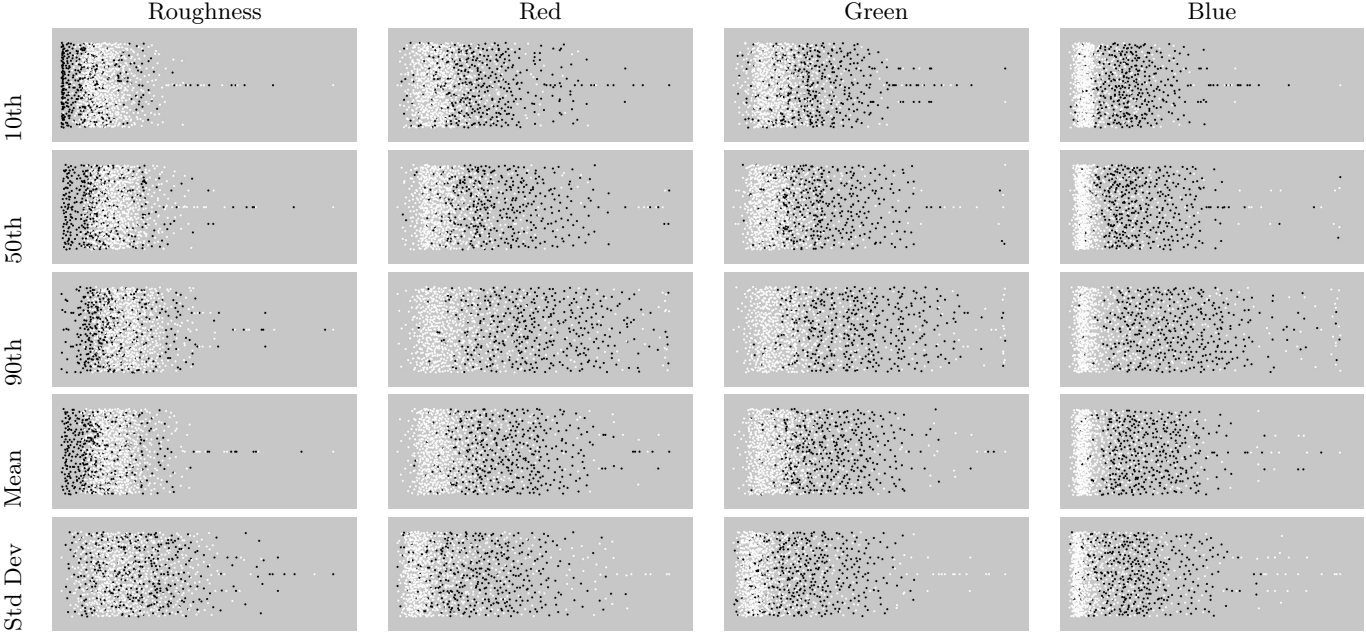
Figure A.5: 1D Plots for segment characteristics - Nijmegen. Values are jittered to emphasise the distribution. Buildings are shown in black and vegetation in white.
