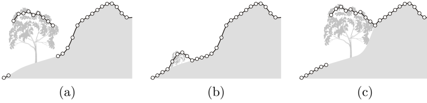
Figure 4.3: Vertical and lateral separation of points, (a) desirable vertical and lateral separation, (b) poor vertical separation, (c) poor lateral separation.
