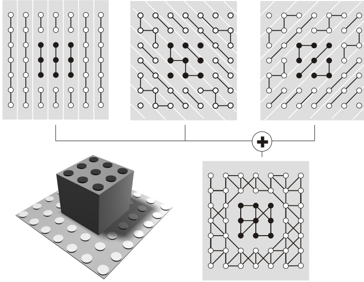
Figure 5.4: Segmenting a point cloud. Two surfaces (the top of the plate and the top of the cube) are segmented using three different profile directions.
