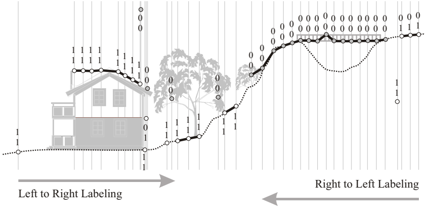
Figure 2.10: Scan labeling algorithm. The solid line indicates points that meet continuity criteria.
