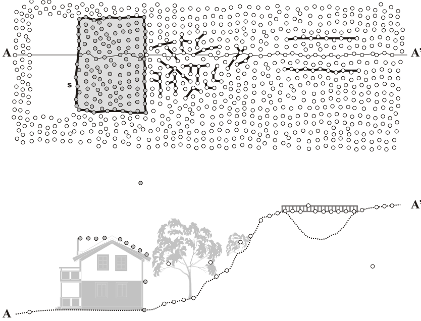
Figure 2.8: Concept of an edge based algorithm.
