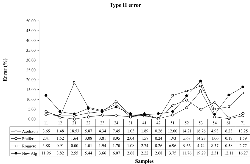
Figure 7.3: Type II errors over the 15 samples
