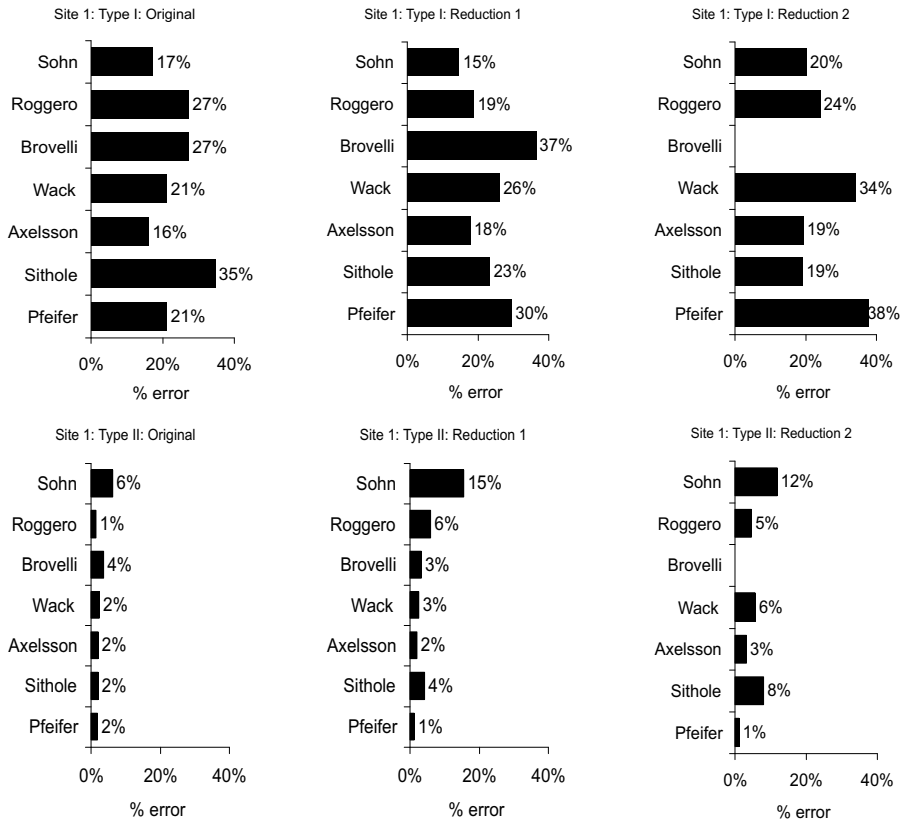
Figure 3.6: Type I and Type II errors of Site 1 vs. resolution.
