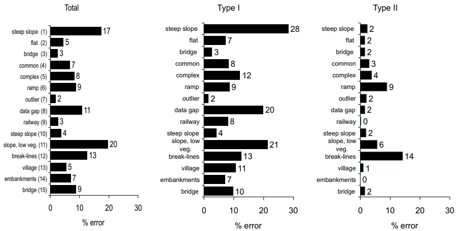
Figure 3.5: The effect of landscape on filter performance
