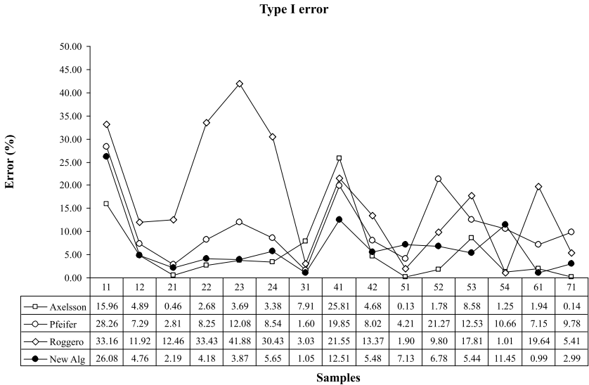
Figure 7.2: Type I errors over the 15 samples
