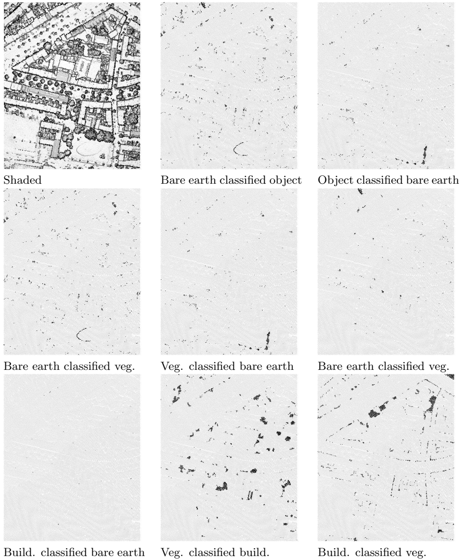
Figure 7.20: Nijmegen test. Depiction of errors in the cross-matrix
