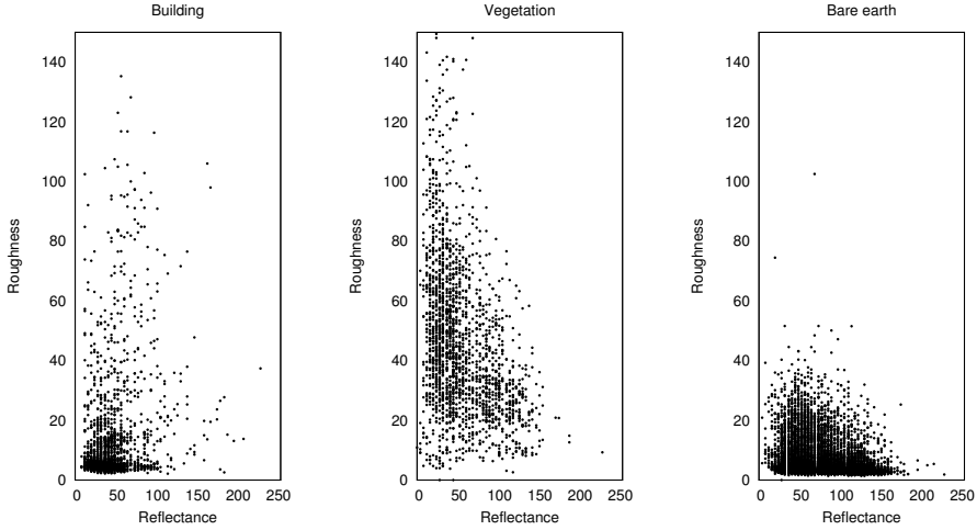
Figure A.2: Scatterplots - Wijhe.
