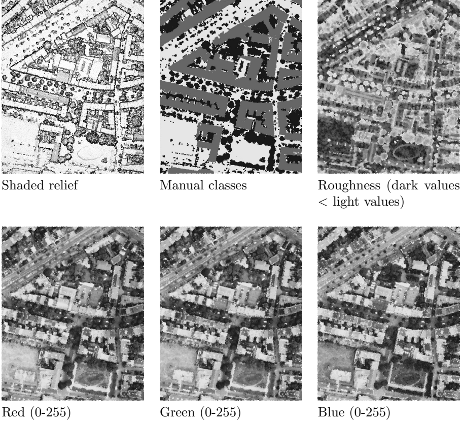
Figure A.3: Nijmegen data characteristics.
