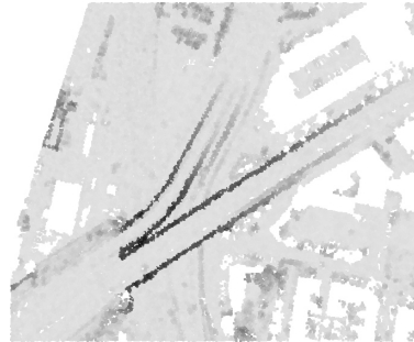
Roughness values are computed for each point in the cloud. Roughness is determined by fitting planes to point neighborhoods and determining the standard deviation of the distance of points from the fitted planes. In the figure above points with a high roughness are shown in dark gray.
