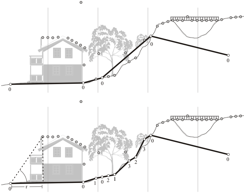
Figure 2.6: Axelsson's progressive TIN densification algorithm. First approximation of the bare earth based on neighborhood minima(top), and subsequent approximations of the bare earth based on angle, \theta and distance to nearest node, r (bottom).
