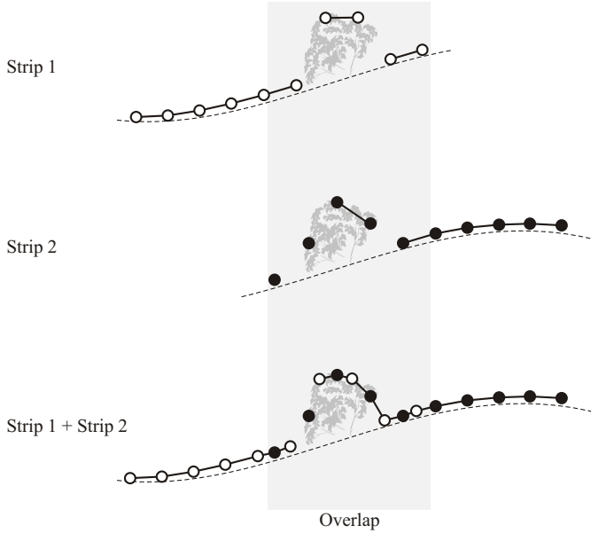
Figure 4.4: Reduction of point spacing in strip overlaps
