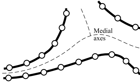
Figure 5.8: Medial axis between curves
