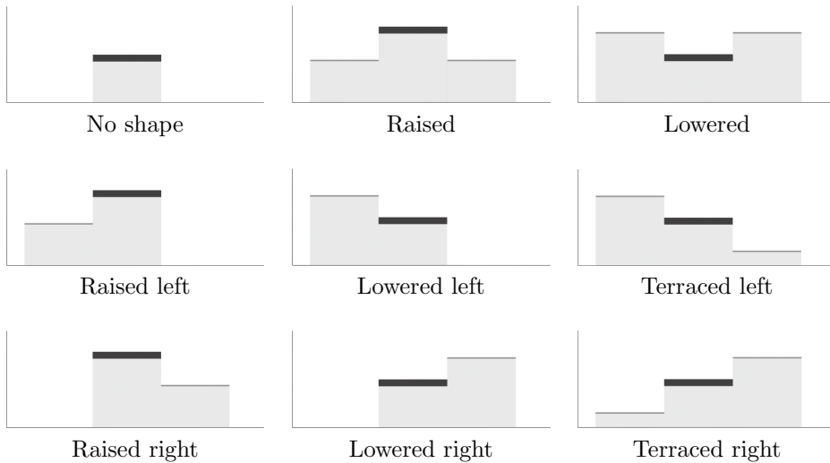
Figure 5.16: Line shapes. Relationships of a line segment (shown by the checkered surface) to neighboring line segments (shown by the gray surfaces)
