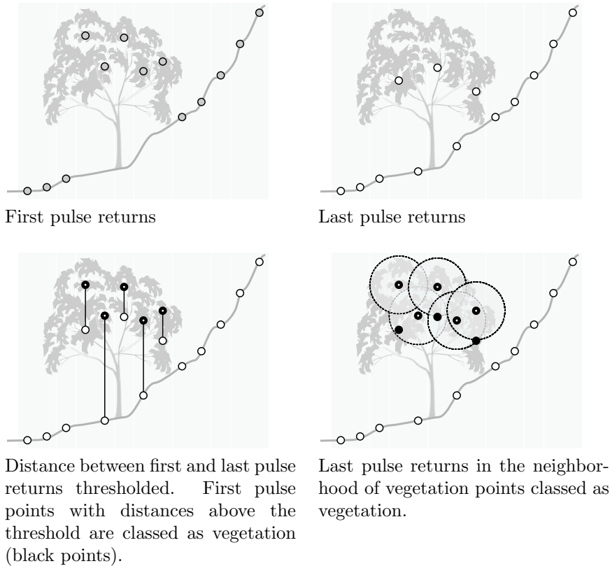
Figure 7.22: Using first pulse returns to classify vegetation in last pulse returns.
