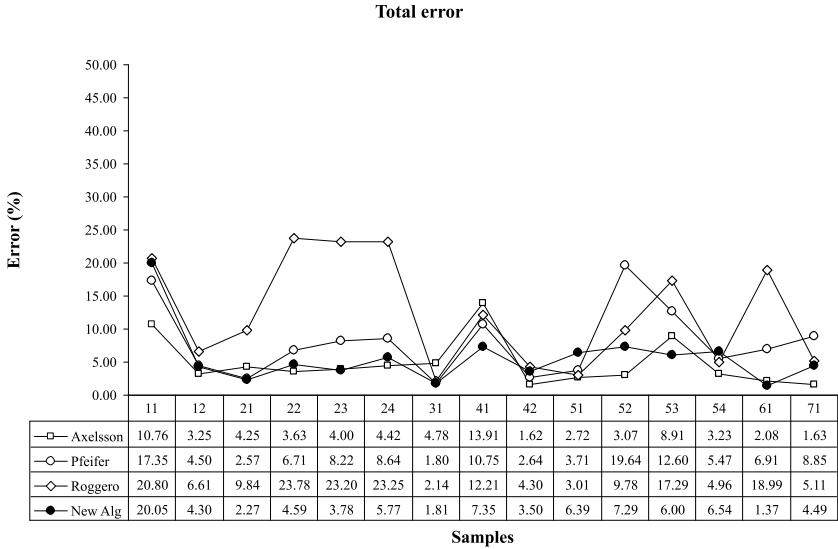
Figure 7.1: Total errors(%) over the 15 samples
