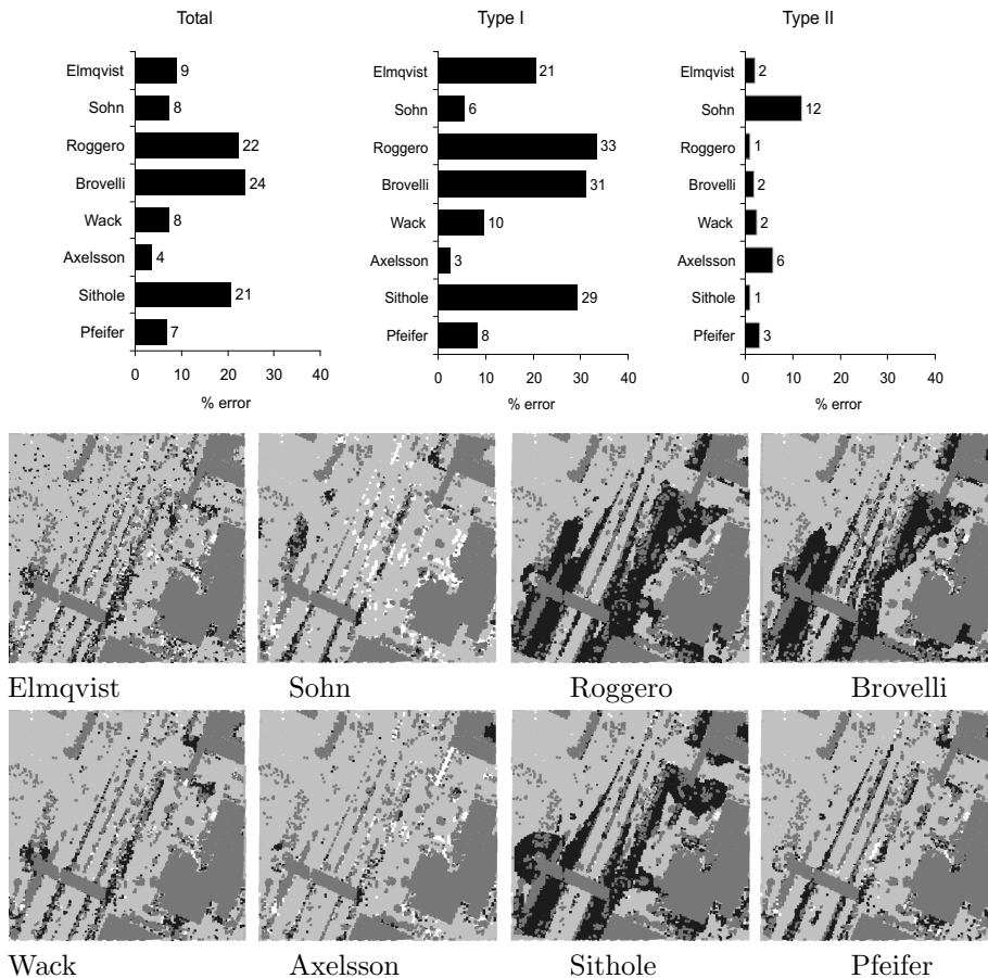
Figure 3.4: Quantitative comparison of site 22
