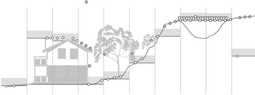
Figure 2.3: Morphological algorithm. White circles are classified as bare earth and gray circles as object.
