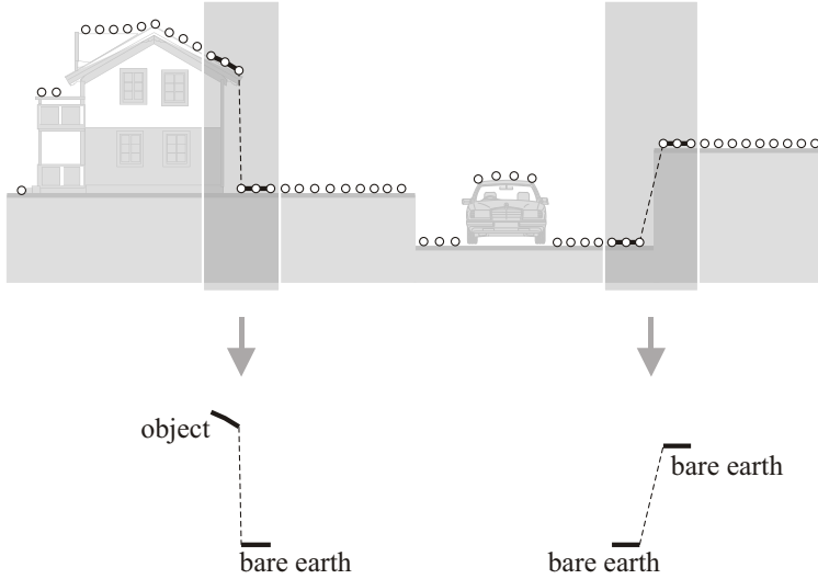
Figure 4.1: Neighborhoods that contain objects and bare earth, and neighborhoods that contain only bare earth are homeomorphic
