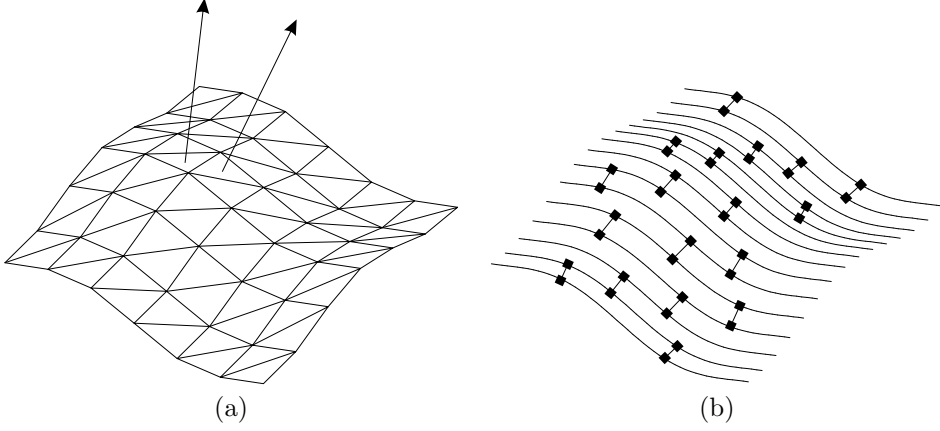
Figure 5.1: Region growing. Region growing in TINs (a), region growing by scan lines (b)
