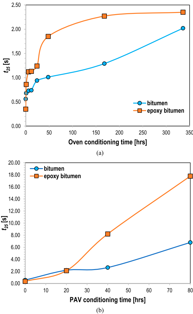
Figure 8. Relaxation time at shear stress level of 25% of the initial stress of binders during (a) oven and (b) PAV age conditioning.
