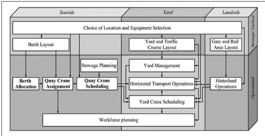
Figure 5. Overview of container terminal operations.
