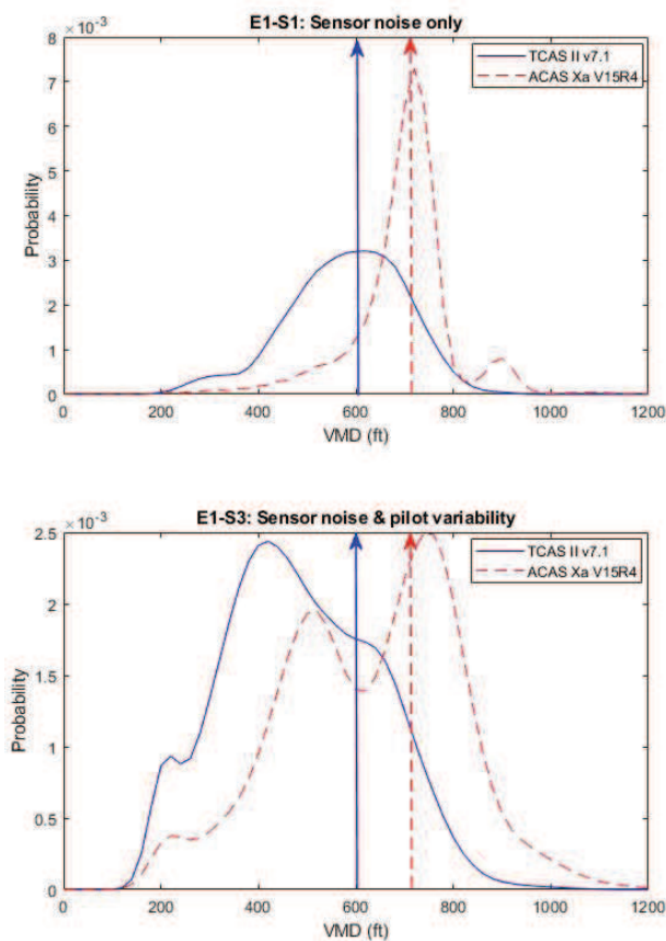
Fig. 5. Deterministic simulation results of encounter scenario E1-D (arrows) and empirical PDFs of the VMD for MC simulation of encounter scenarios E1-S1 (top) and E1-S3 (bottom) for TCAS II v7.1 and ACAS Xa V15R4.
