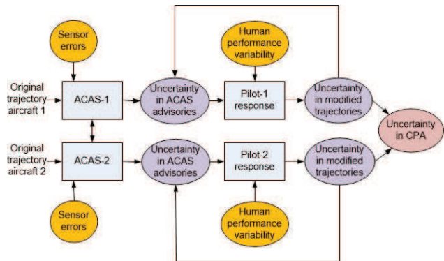
Fig. 1 Sources of uncertainty in evaluation of ACAS in an encounter of an aircraft pair
