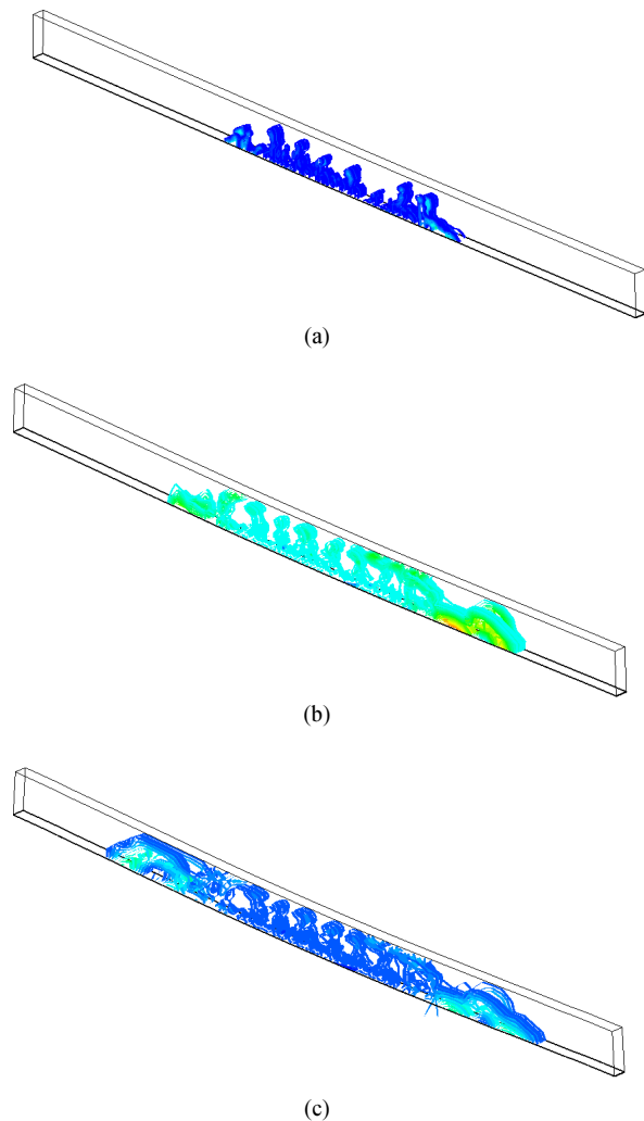
Fig. 13. Crack propagation in glass, axonometric isocurves at selected deflection amplitudes for the FE numerical model (ABAQUS (Simulia 2012)) (a) \mu_{max} = 5\text{mm} ; \mu_{max} = 15\text{mm} ; (c) \mu_{max} = 25\text{mm}
