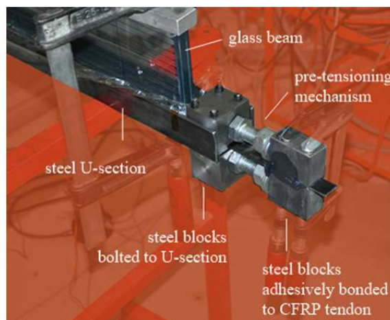
Fig. 2. Photograph of the post-tensioning rig (side A)
