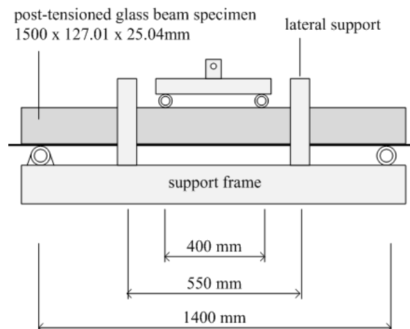
Fig. 4. Schematic representation of the four-point bending test setup (front view)
