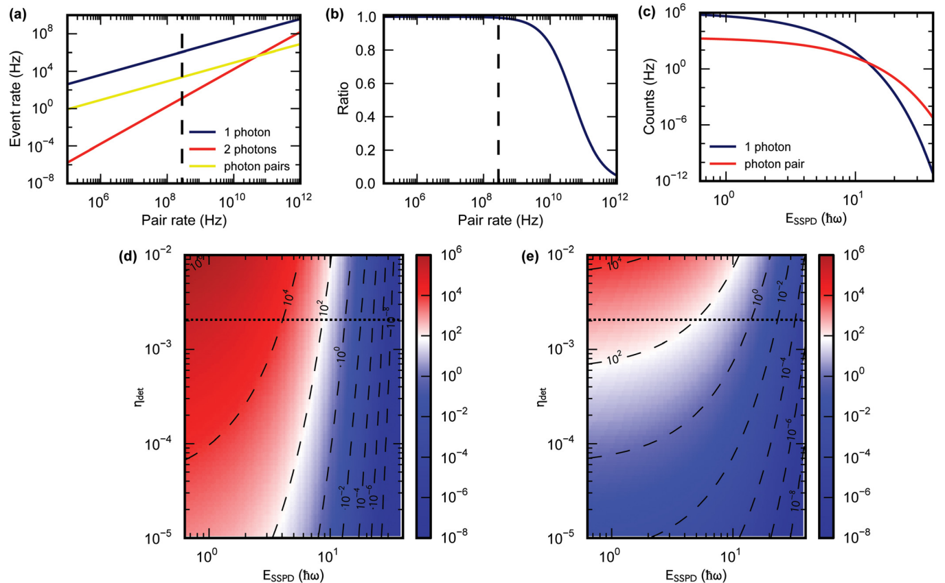
FIG. 1. (a) The number of 1-photon, accidental 2-photon, and correlated 2-photon absorption events as a function of the pair production rate with \eta_{abs} = 2 \times 10^{-3} and bin-size ( dt ) of 20 ps. The dashed line indicates the pair production rate in this experiment. (b) The ratio of correlated 2-photon events versus total (correlated and coincidental) 2-photon events as a function of pair production rate. (c) Count-rates caused by 1 photon events and by correlated 2-photon events as a function of SSPD energy scale in units of the single photon energy. (d) and (e) Single-photon (d) and 2-photon (e) count rates as a function of absorption probability \eta_{abs} and SSPD energy scale. Line-cuts along the dotted lines give (c).
