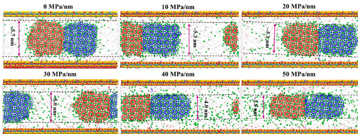
Fig. 12. Snapshots of hydrate dissociation in 10.0 ns in clay pore for the PHS system at 287 K for different pressure gradients.
