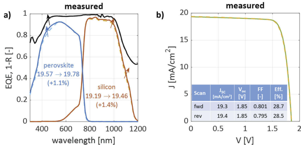
Fig. 2. a) Measured EQE of top and bottom cell (blue and red lines) and 1-R (black line) for tandem with gentle texture (solid lines) and flat reference (dashed lined). b) Measured JV-curve in forward (green) and reverse (orange) scan direction of tandem with gentle texture. The inset shows the measured external parameters.
