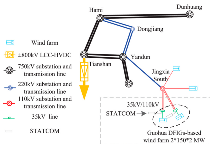
Figure 5. Single line diagram of the wind power system in Xinjiang [5].
