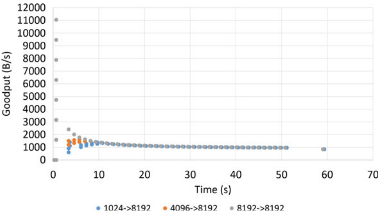
Fig. 7.4 Goodput of the TCP session for different initial CWND sizes for 50 kB data transfer
