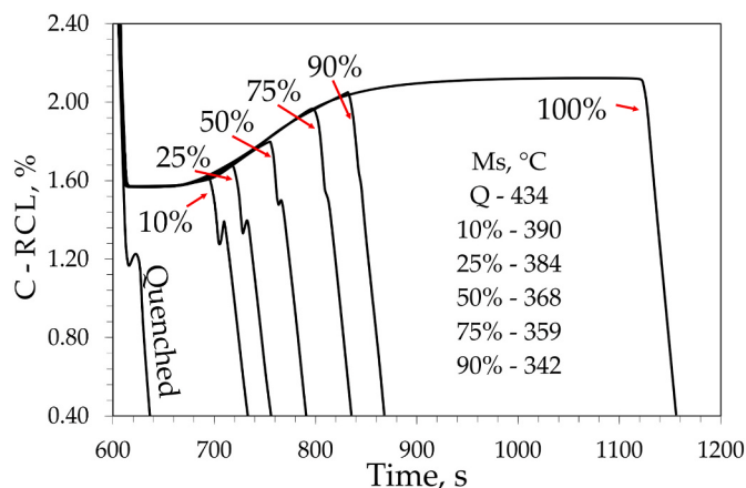
Fig. 1. M_s changes with increasing degree of bainitic transformation at 450 °C; RCL - relative change in length.
