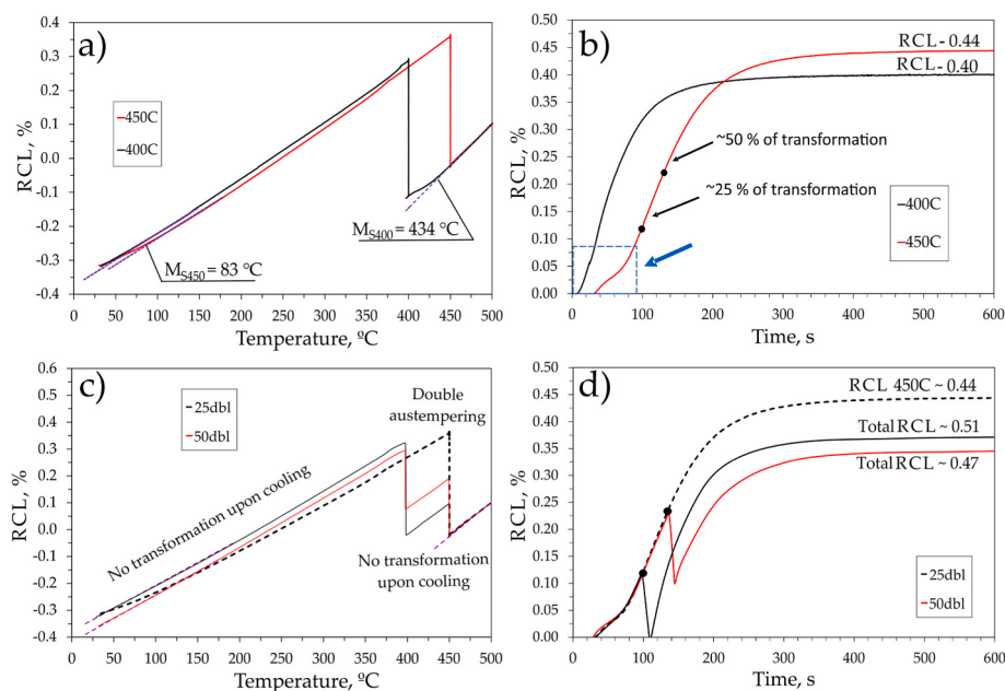
Fig. 3. The dilatometric curves of samples 450C and 400C: (a) cooling; (b) austempering; and samples 25dbl and 50dbl: (c) cooling; (d) double austempering; C-RCL - corrected relative change in length; dashed lines in (c) and (d) represent results for the 450C sample.
