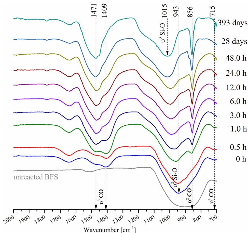
Fig. 6 FT-IR spectra of powdered AAS exposed to accelerated carbonation (Color figure online)
