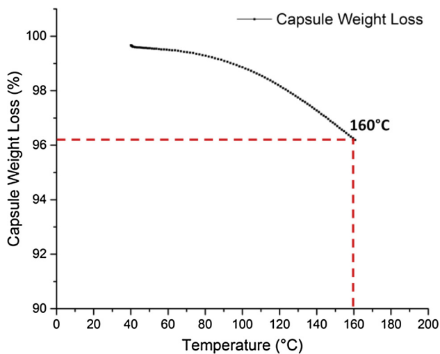
Fig. 11. Thermogravimetric analysis.
