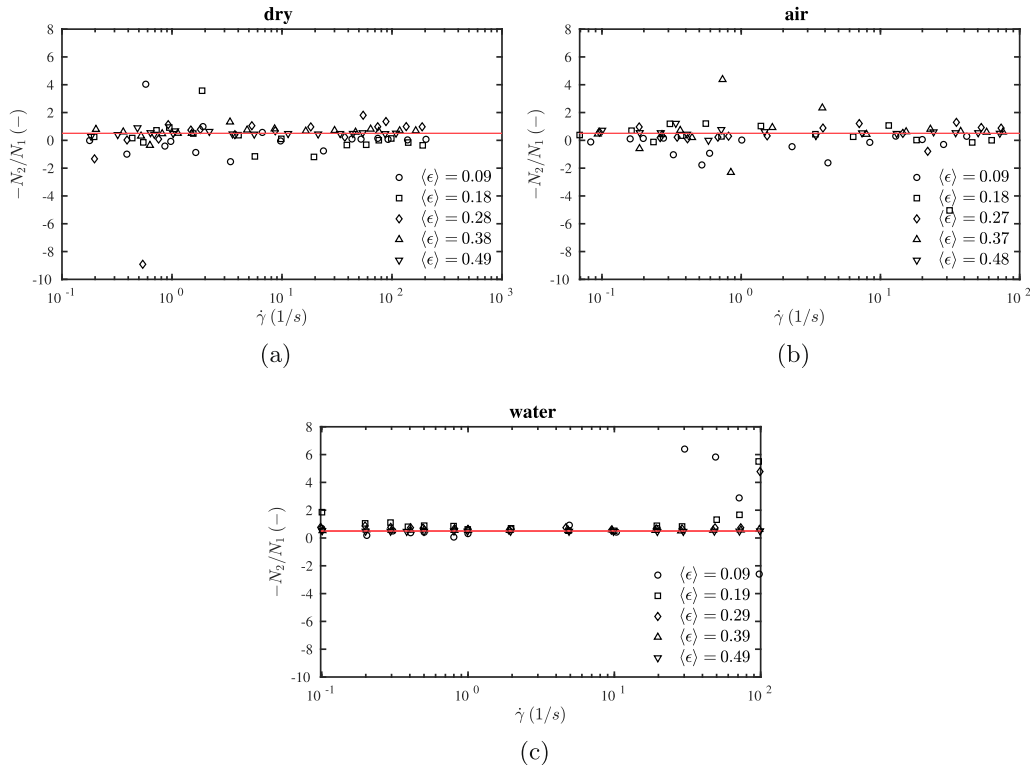
Fig. 15. Particle normal stress ratios for (a) granular (b) air and (c) water. cases. The red line indices N_2/N_1 = -1/2 , as observed for many other rod-like systems. (For interpretation of the references to color in this figure legend, the reader is referred to the web version of this article.)
