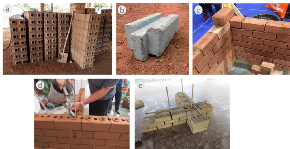
Figure 3. A collection of various compressed stabilized earth block (CSEB) and interlocking stabilized soil block (ISSB). (a) ISSB in Uganda (model 'Tanzania'); (b) interlocking Hydraform ISSB Uganda; (c) rectangular loam bricks for Mali; (d) Interlocking blocks Thailand; (e) adobe blocks for walls El Salvador. Source: Bredenoord.
