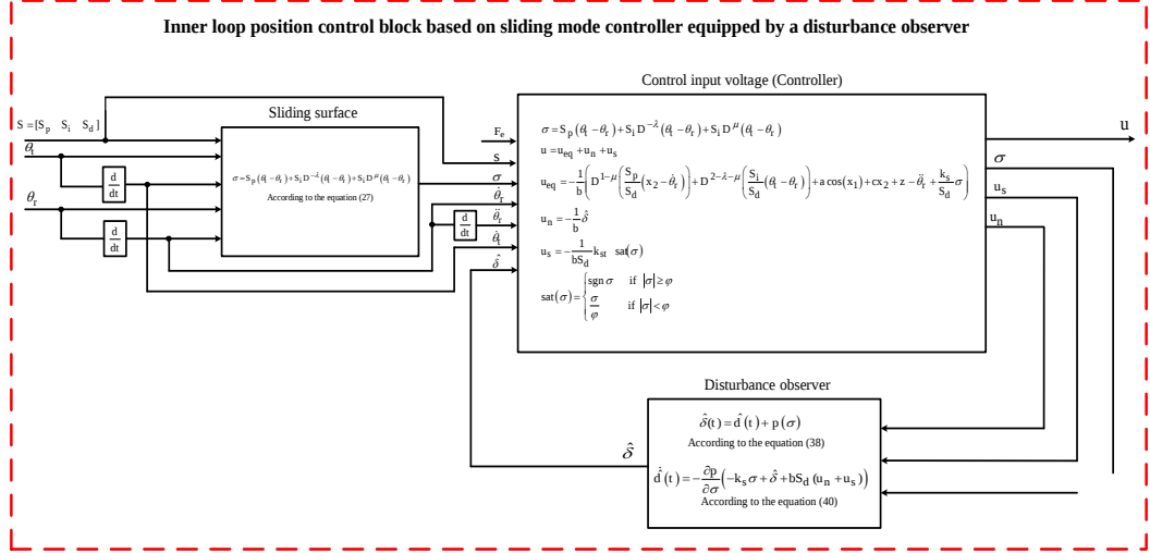
Fig. 5. Inner loop position control block based on fractional order sliding mode controller equipped with a disturbance observer.
