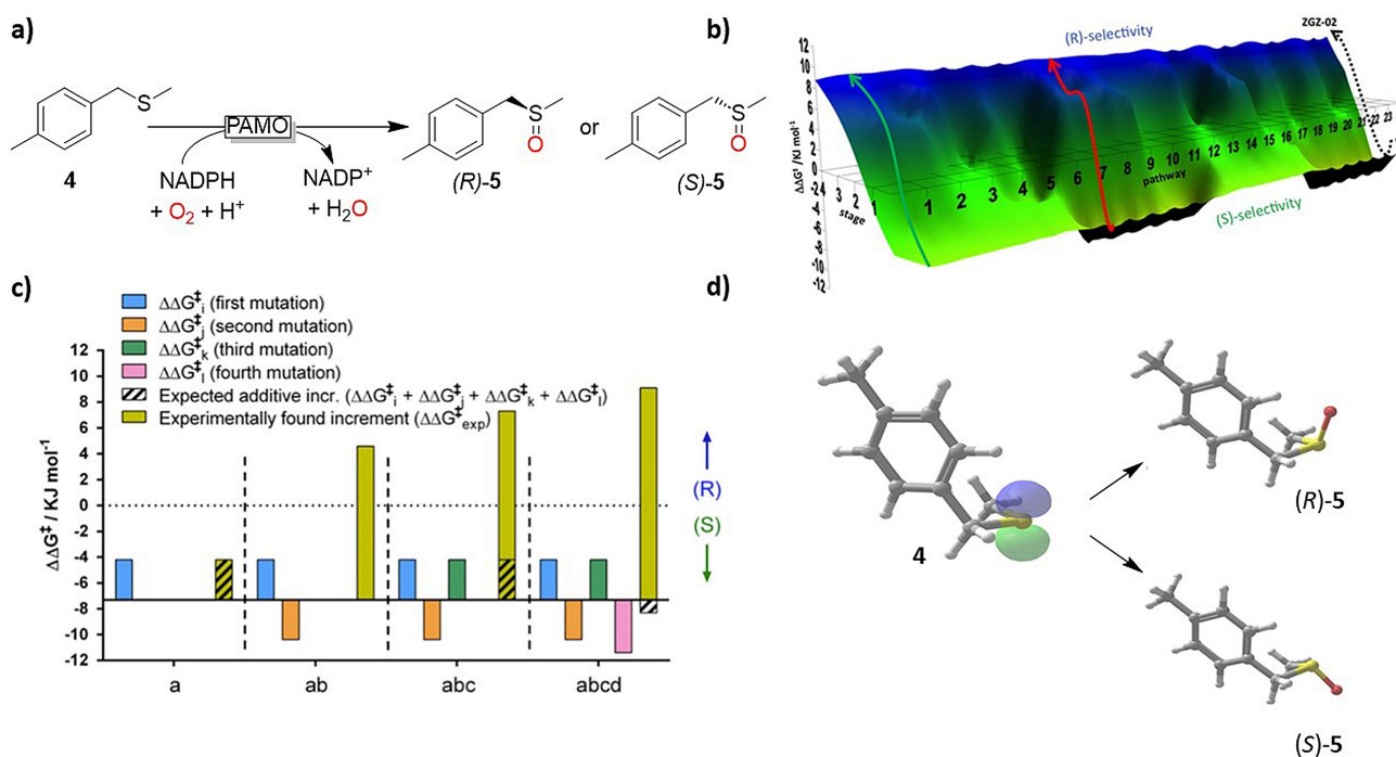
Figure 4. Directed evolution of the Baeyer–Villiger monooxygenase PAMO as the catalyst in the successful quest to invert the sulfoxidation enantioselectivity of a prochiral thioether. [38] a) Reaction of thioether 4 as prochiral substrate. b) Fitness pathway landscape based on mutational data derived from complete deconvolution of the best (R)-selective PAMO mutant I67Q/P440F/A442N/L443I. c) Typical deconvolution data showing the effects of the four single mutations. d) Model indicating which lone-electron pair (blue or green) is closest to the active PAMO oxidant FAD-OOH, therefore leading to the (R)- or the (S)-sulfoxide, respectively. With permission from American Chemical Society.
