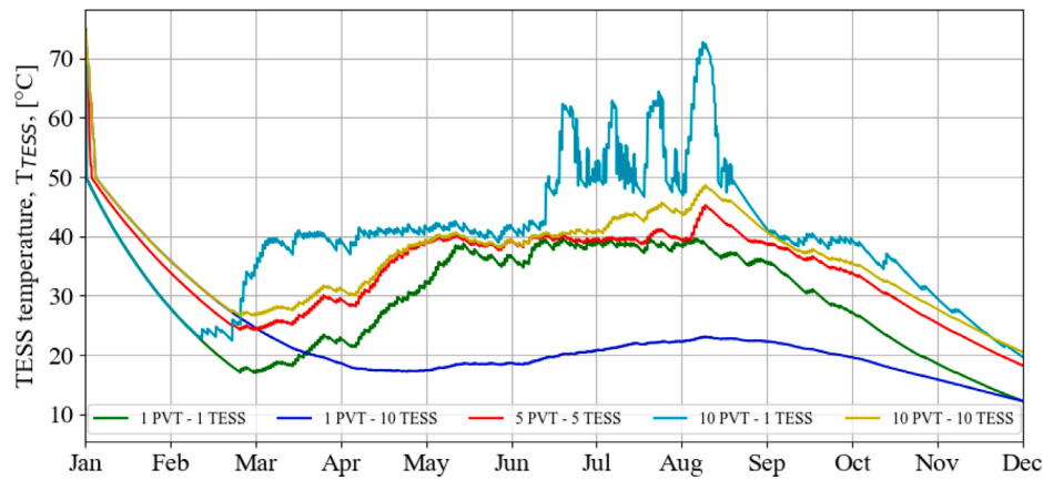
Fig. 15. Temperature in the TESS during the year for different numbers of PVT modules and TESS volumes in Scenario 3.
