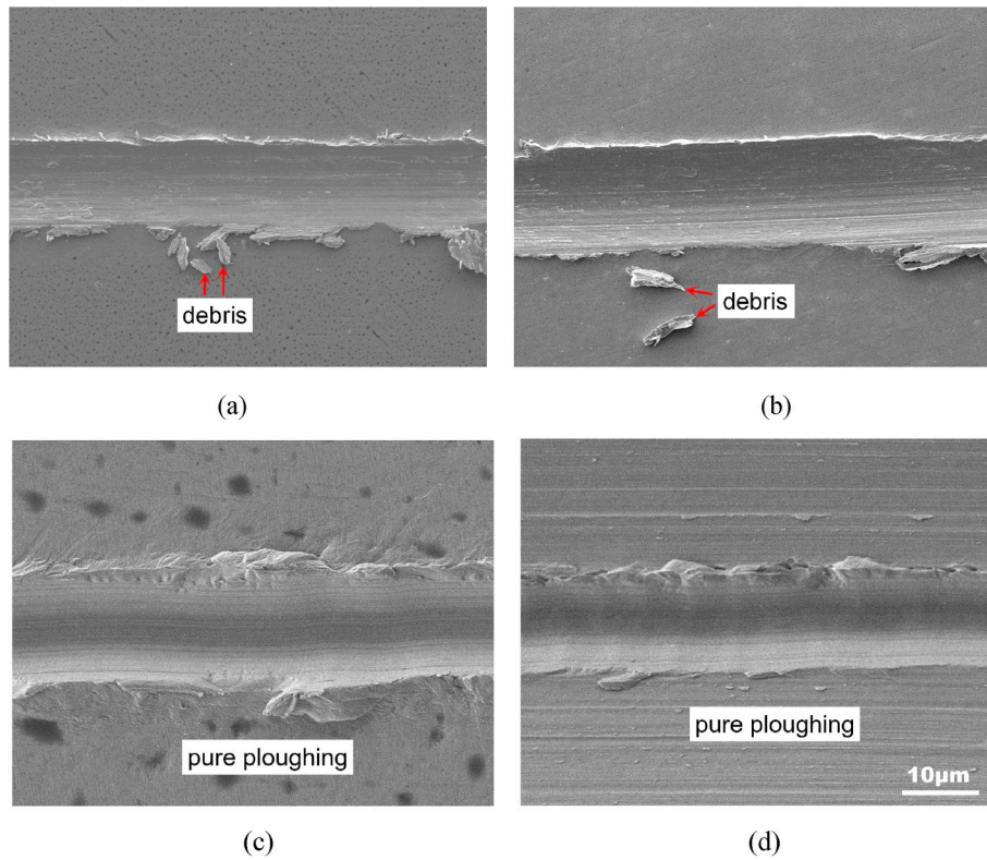
Fig. 14. Scratch tracks of Ti-10V-1Fe-3Al alloy by the small indenter with 0.3 N following pre-scratching under 0 N, 10 N loads (a)-(b): 900 °C/15 min + Q+550 °C/15 min, (c)-(d): 900 °C/15 min + 700 °C/10 min.
