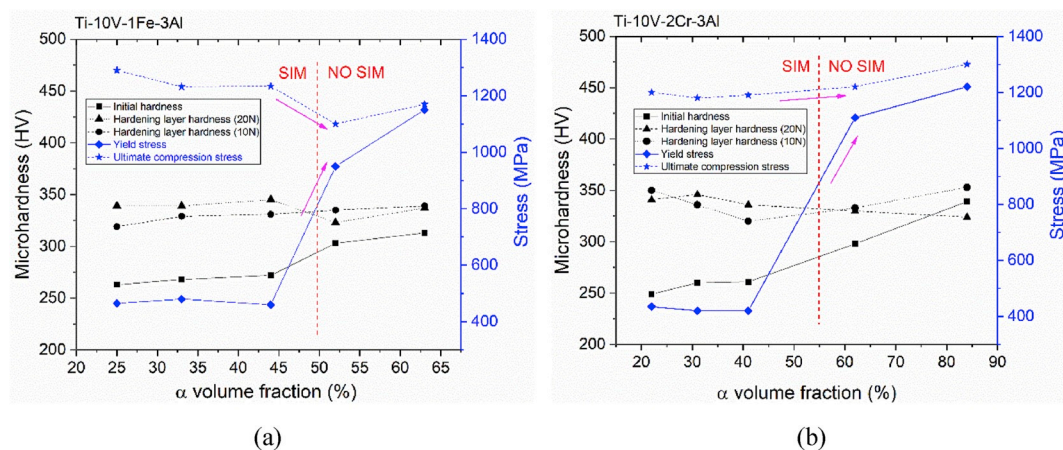
Fig. 6. Various parameters as a function of \alpha volume fraction (a) Ti–10V–1Fe–3Al alloy solution treated in \alpha + \beta phase field, (b) Ti–10V–2Cr–3Al alloy solution treated in \alpha + \beta phase field.
