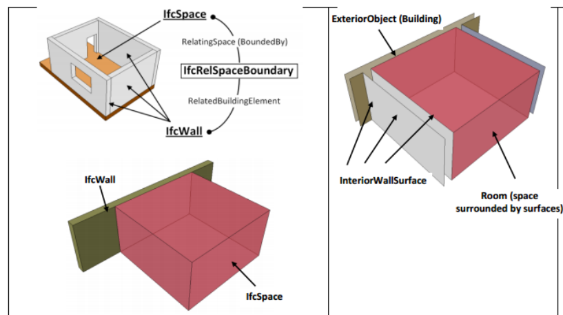
Figure 4: Conceptual difference between IFC (left) and CityGML LOD4 (right) for modelling interiors (courtesy Filippo Mortari)
