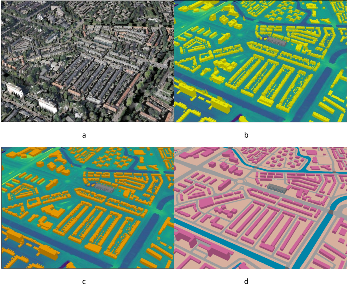
Fig. 4. Obstacle models (a) Model 1: DSM produced with first return points of AHN3 (b) Model 2.1: DTM plus buildings with rooftop geometry (c) Model 2.2: DTM plus buildings extruded with mean height of rooftop point (d) Model 3: TOP10NL dataset
