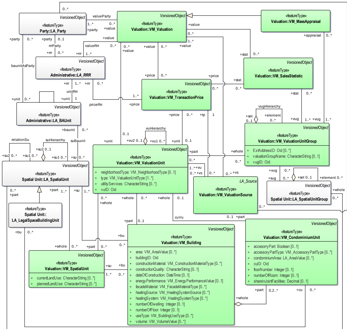
Fig. 2. The spatial part of the LADM Valuation Information Model
