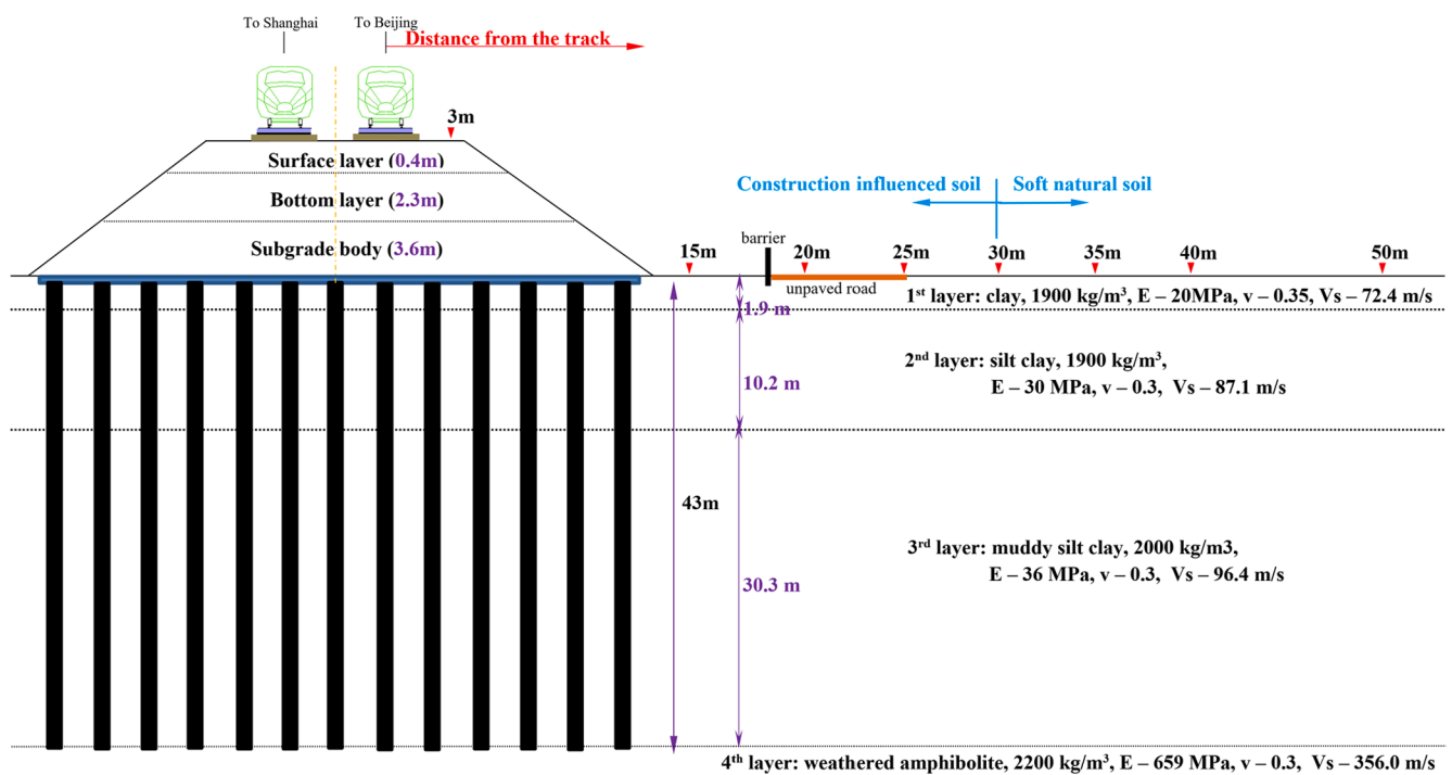
Fig. 2. Schematic diagram of the cross section and measurement points at various distances from the track (E – Young’s modulus, ν – Poisson’s ratio, Vs – shear wave velocity).
