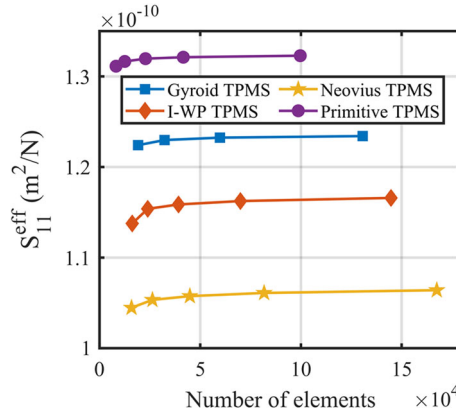
Fig. 5 Mesh sensitivity analysis of effective compliance coefficient S_{11}^{\text{eff}} for Schoen Gyroid, Neovius, Schoen IWP, and Schwarz primitive-based electrostrictive composite's RVE
