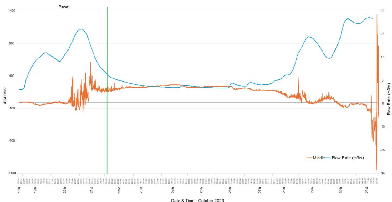
Figure 3. Strain plotted against time for the middle fin during storm Babet
