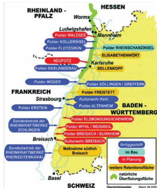
Figure 28 Overview of German and French Room for the River measures along the Upper Rhine (LUBW) and along the Lower Rhine (Umweltbericht NRW, 2009)
