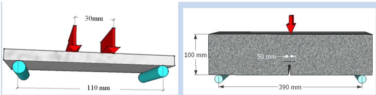
Fig. 2. Flexural tests: a) four-point bending test, b) three-point bending test on notched sample.
