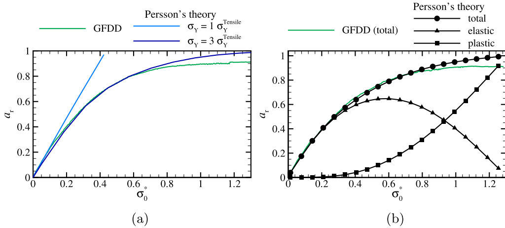
Fig. 6. Relative contact area a_r calculated using GFDD and modified-Persson's theory. In the latter, yield strength \sigma_Y = \sigma_Y^{\text{Tensile}} and 3 \sigma_Y^{\text{Tensile}} were applied as an input.
