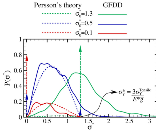
Fig. 8. Probability distribution of the contact stress \sigma^* at three instances of loading, \sigma_0^* = 0.1, 0.5 , and 1.3 , for an indenter with \bar{h} = 0.001 \mu\text{m} and \epsilon_f^{-1} = 64 .
