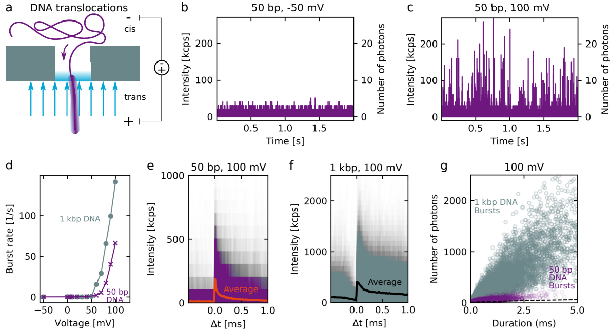
Figure 4. Voltage Driven DNA Translocations a: DNA can be driven through a ZMW by a voltage that is applied across the membrane, where individual translocation events are recorded optically. b: When a negative bias of -50 mV is applied to the trans side, no translocations of 50 bp double-stranded DNA labeled with the intercalating dye Yoyo1 were observed through the 59 nm by 47 nm oval pore. c: At 100 mV, however, many events were detected. Notably, these DNA translocations are well resolved despite the low salt, low bias voltage, short DNA length, and large pore size. d: Burst rate versus driving voltage for two different DNA lengths. The error bars (standard deviation due to the statistical error) are smaller than the markers. e: Average shape from 2000 individual fluorescence bursts for 50 bp DNA. f: Same for 1 kbp DNA. g: Photons per burst vs. burst duration at 100 mV bias. Bursts below the dashed line are ignored in further analysis. Bursts from longer DNA involved more photons. The full dataset is displayed in supplementary figure A4 together with the FCS data for the different voltages. DNA concentrations were 5 ng/ \mu l in the reservoir cis side. Binning for the plots in b and c was 100 \mu s and 10 \mu s for e and f.
