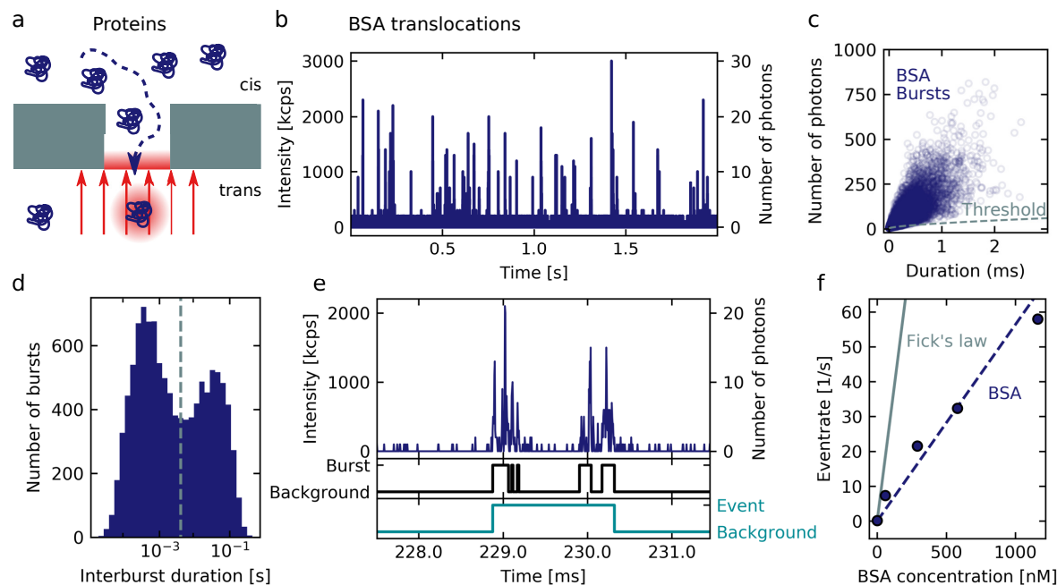
Figure 3. Diffusion Driven Protein Translocations a: Schematic of protein translocations. The translocation of fluorophore-labeled proteins can be studied using Pd ZMWs, without requirements for a specific salt concentration or a bias voltage. b: Time trace of 290 nM bovine serum albumin (BSA) labeled with Alexa647 that freely translocate through a 43 nm pore. c: Number of photons per burst vs. burst duration. Bursts below the threshold likely do not involve a fluorophore-labelled protein and were removed. The full scatter plot is shown A3 together with the FCS signal for different BSA concentrations. d: Number of bursts versus interburst duration. Two populations can be identified. The populations with the lower interburst duration is attributed to re-entries of the same protein to the laser focus. e: One example event that illustrates how multiple bursts are combined to individual long events when their interburst duration is below a certain threshold time (here 4 ms). f: Translocation rate versus BSA concentration. Error bars (standard deviation due to the statistical error) are smaller than the data markers. The solid grey line shows the prediction by Fick's law of diffusion. The dashed line is a linear fit to the data. Binning in b and e is 10 \mu s.
