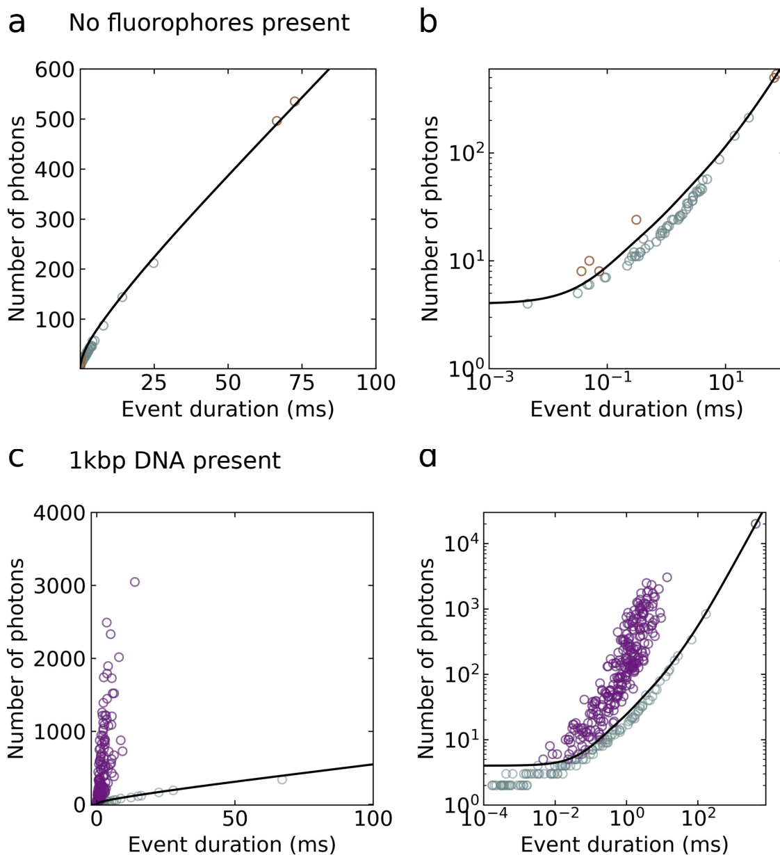
Figure A1. a,b: Scatter plots of the bursts detected by the spike-detection algorithm from the dataset in figure 2b. If a burst involves less spikes than the empirical threshold (black line) it is sorted out (grey). In the case of panel a/b, no fluorophores were present in the system, so all remaining bursts (brown) are likely false positives. c,d: Scatter plots from 1 kbp DNA translocation data at 60 mV, from figure 4. The scatter plots show two populations, the DNA bursts (purple) and the background bursts (grey) that lie below the threshold (black line).
