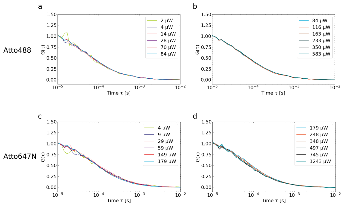
Figure A5. a,b: Normalized FCS curves for Atto488 measured in open solution for laser powers below and above 84 \mu\text{W} . c,d: Normalized FCS curves for Atto647N measured in open solution for laser powers below and above 179 \mu\text{W} . The fact that there is no significant shift visible for varying laser power, shows that bleaching is not a dominant process in these regimes.
