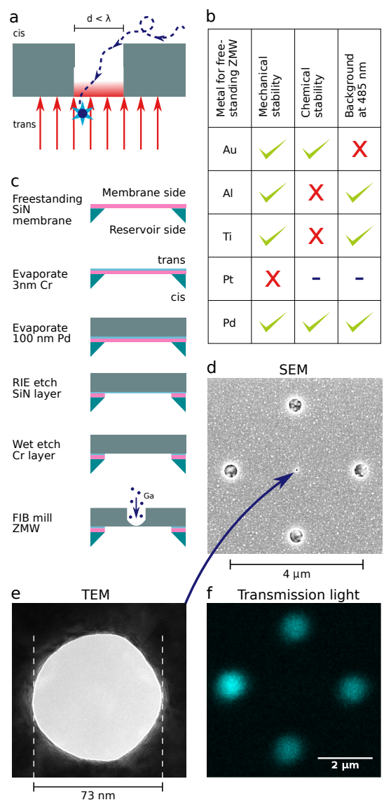
Figure 1. Fabrication of Pd ZMW a: A zero-mode waveguide is a sub-wavelength aperture in a metal film. They have the property to block impinging light such that an evanescent field is generated in the pore with an exponential intensity decay. When a fluorophore traverses the nanohole from the cis side towards the laser-illuminated trans side (dashed line), it can be detected by its fluorescence. b: Various metals were tested for their suitability for ZMW detection of translocating single molecules. Whereas gold produced a background in the 550nm range when illuminated with a 485 nm laser, aluminum and titanium were not stable in chlorine-based solutions, see SI Figure A2. When platinum was deposited, its mechanical stress made it impossible to fabricate free-standing membranes. Only palladium fulfilled all requirements. c: Freestanding Pd films were made by e-beam evaporation and support layers were subsequently removed by etching. Local ZMW and marker structures were fabricated using Focused Ion Beam Milling. d: SEM image of the marker structures, that allow a localization of the nanohole. e: TEM image of the central nanopore in d. f: Transmission light image of the markers.
