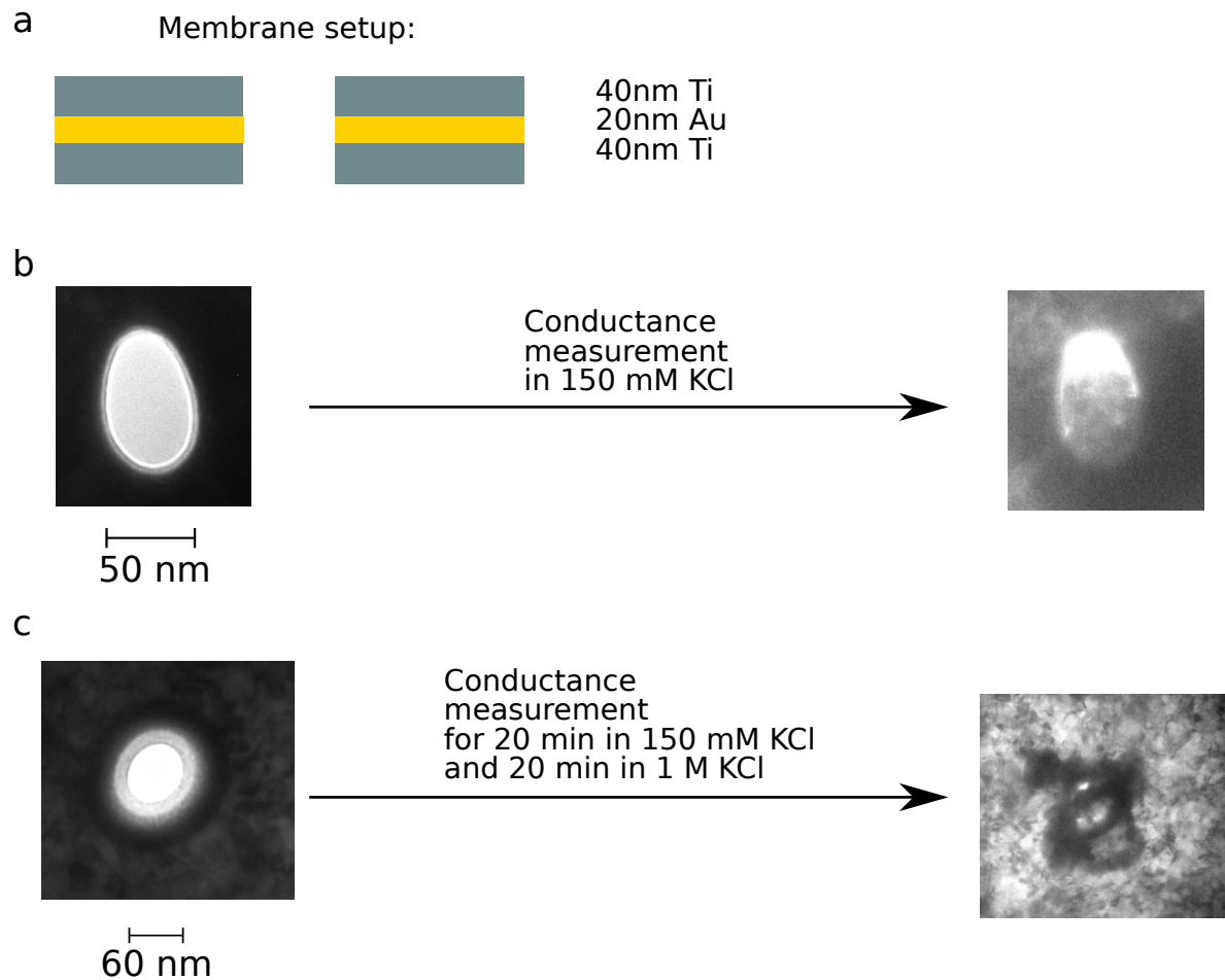
Figure A2. a: During the search for suitable materials we used a Ti, Au, Ti sandwich structure. After fabrication pores had a clear shape (b,c, left side) but after conductance measurements in KCl the pore structure changed completely (b,c, right side). We concluded that these Ti-Au-Ti sandwich structures were not usable for experiments in liquid.
