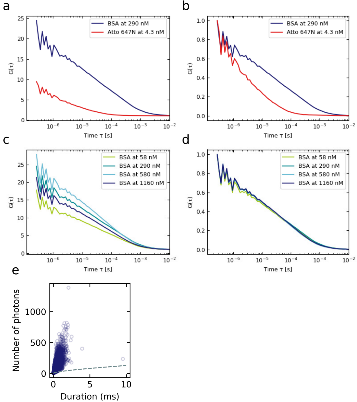
Figure A3. a: FCS curves for BSA vs. Atto647N translocation events. The difference in timescales, due to slower diffusion for BSA, is reflected by a shift of the FCS curve along the x axis. b: Normalized FCS curves from a. c: FCS curves for BSA at different concentrations. d: Normalized FCS curves from c. The normalised FCS curves fall upon each other, as no mutual interaction is expected for BSA. e: Scatter plot of the full dataset shown in figure 3c.
