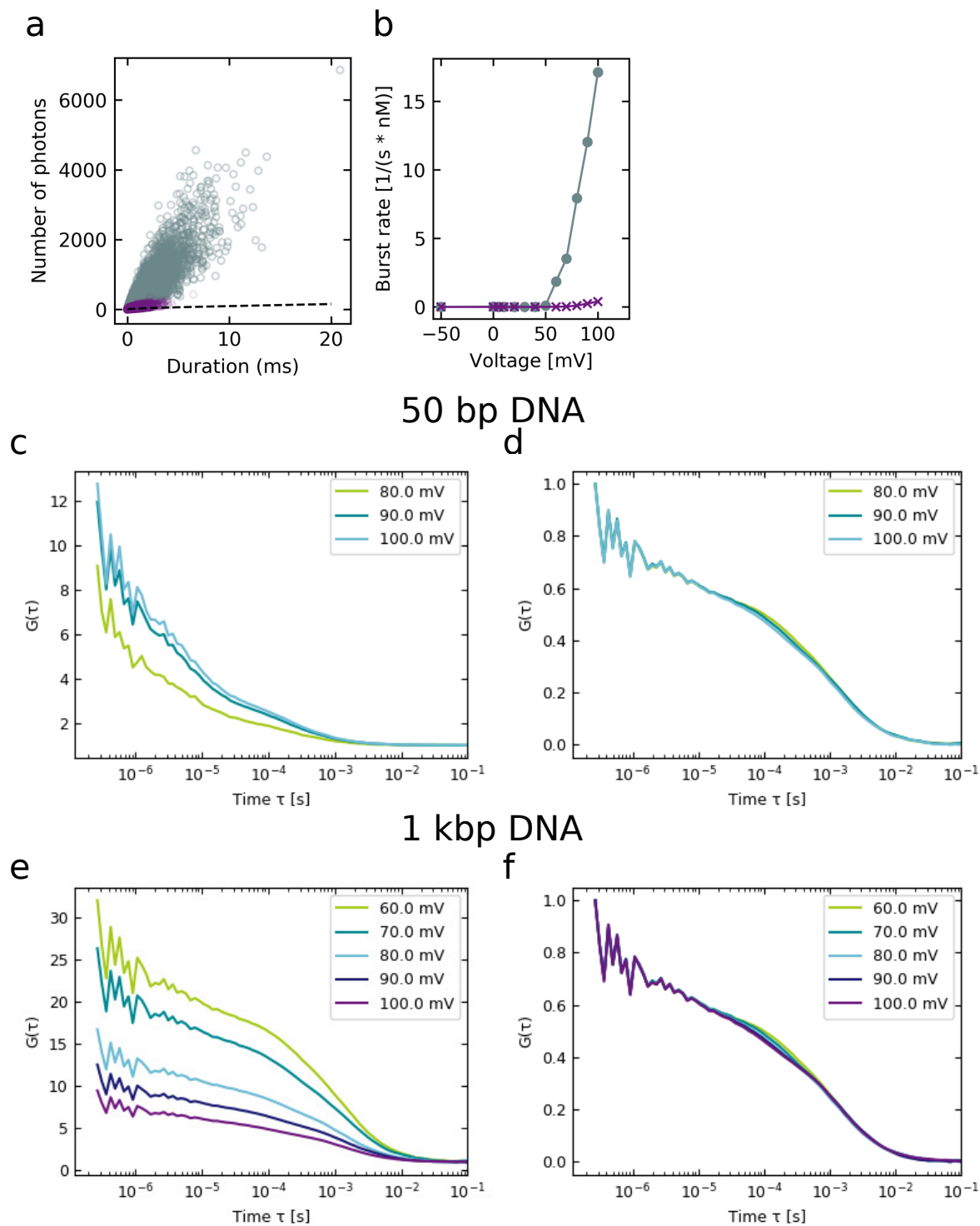
Figure A4. a: Scatter plot of the full dataset shown in 4g. b: Burst rates shown in figure 4d, normalized to molarity. c: FCS curves of 50 bp DNA at different voltages. d: Normalized FCS curves from c. e: FCS curves of 1 kbp DNA at different voltages. f: Normalized FCS curves from e.
