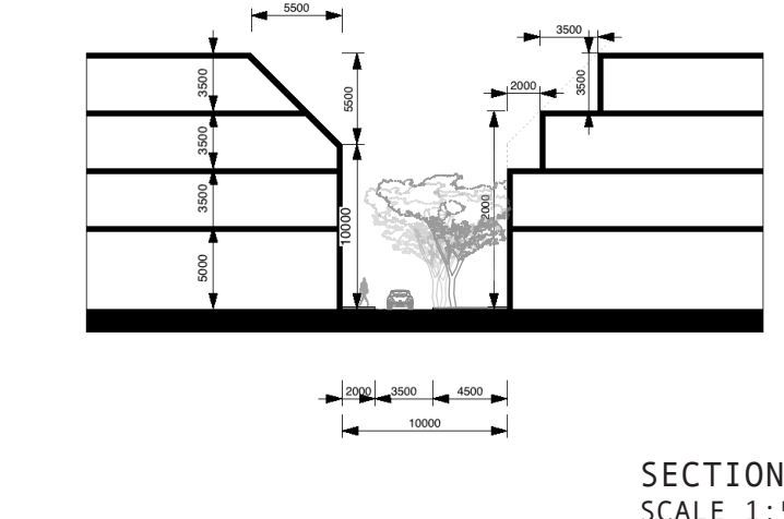
SECTION BB SCALE 1:500
