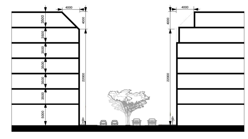
SECTION EE SCALE 1:500
