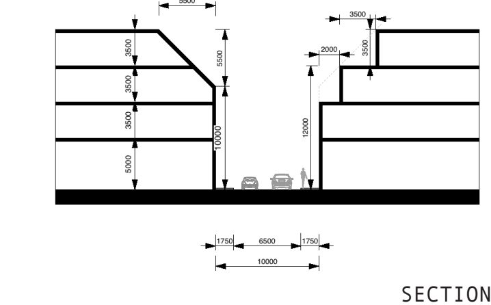
SECTION CC SCALE 1:500
