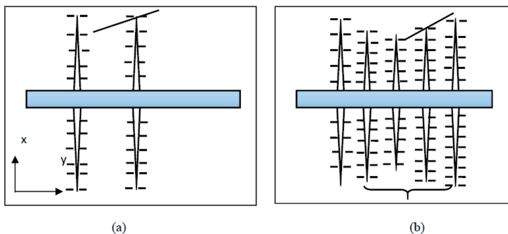
Figure 3. The illustration of discretion of fractures: (a) multi-stage fracturing (b) multi-cluster fracturing.
