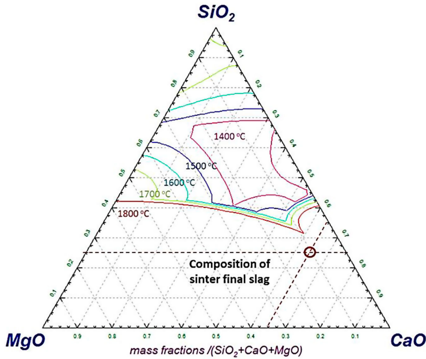
Figure 7. Phase diagram ( \text{SiO}_2 -CaO-MgO-(6.25%) \text{Al}_2\text{O}_3 ) with liquidus temperature projections.
