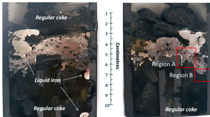
Figure 4. Photographs of two halves of quenched iron ore sinter bed at 1550^\circ\text{C} .
