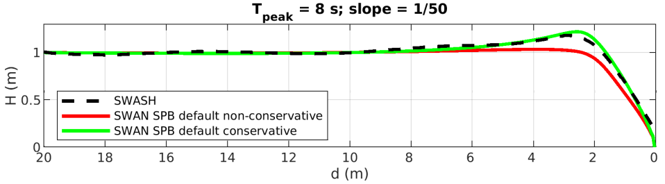
Figure 4.13: Spatial evolution of wave height for an input spectrum with incoming significant wave height of 1 m and T_{peak} = 8 s over a constantly sloping bathymetry with a slope of 1/50. Different lines indicate the outcome of the phase-resolving model SWASH (black dashed), and spectral model SWAN with default SPB settings without energy conservation correction (red), and spectral model SWAN with default SPB settings with energy conservation correction (green).
