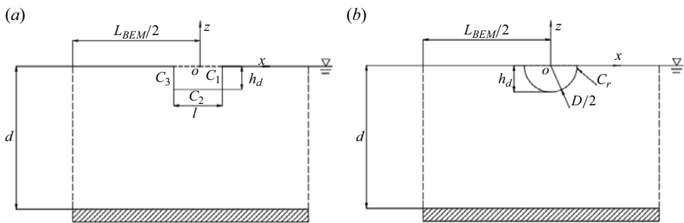
Figure 3. Domain and coordinate system in the diffraction-modified Stokes drift model for the two objects considered, also showing object dimensions. Results are shown for a (a) rectangular box (RB) and (b) RO.
